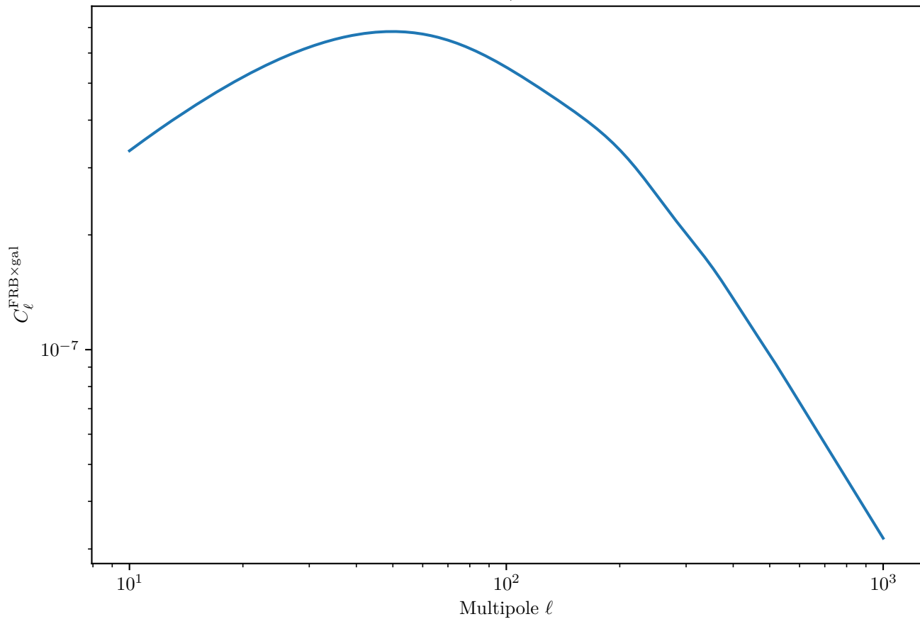
LSST Y10 FRB×Galaxy Cross-Correlation (Neutron Stars, Deep Survey, Galaxy Bin 8)
