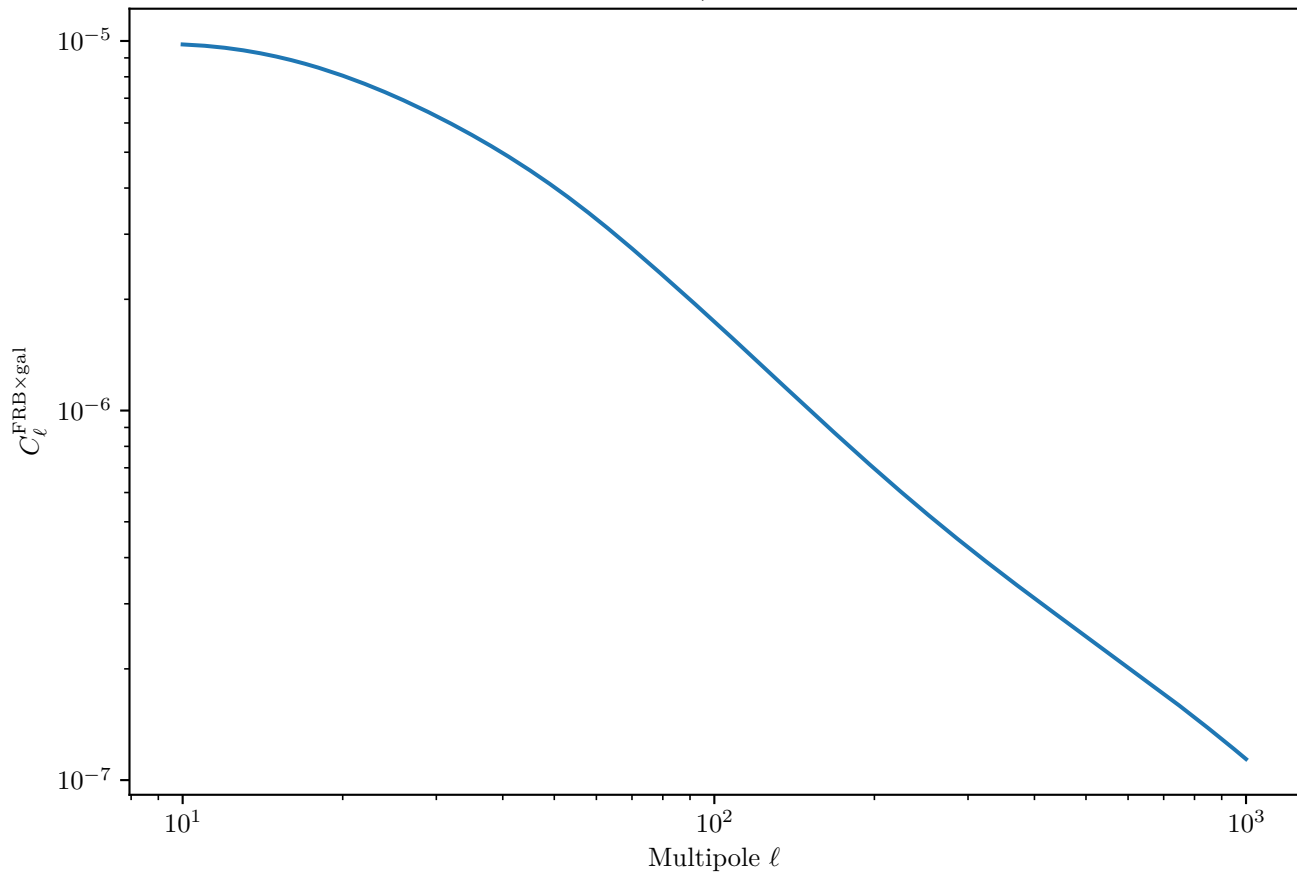
LSST Y10 FRB×Galaxy Cross-Correlation (Neutron Stars, Shallow Survey, Galaxy Bin 1)
