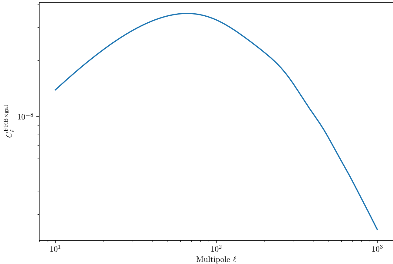
LSST Y10 FRB×Galaxy Cross-Correlation (Neutron Stars, Shallow Survey, Galaxy Bin 10
