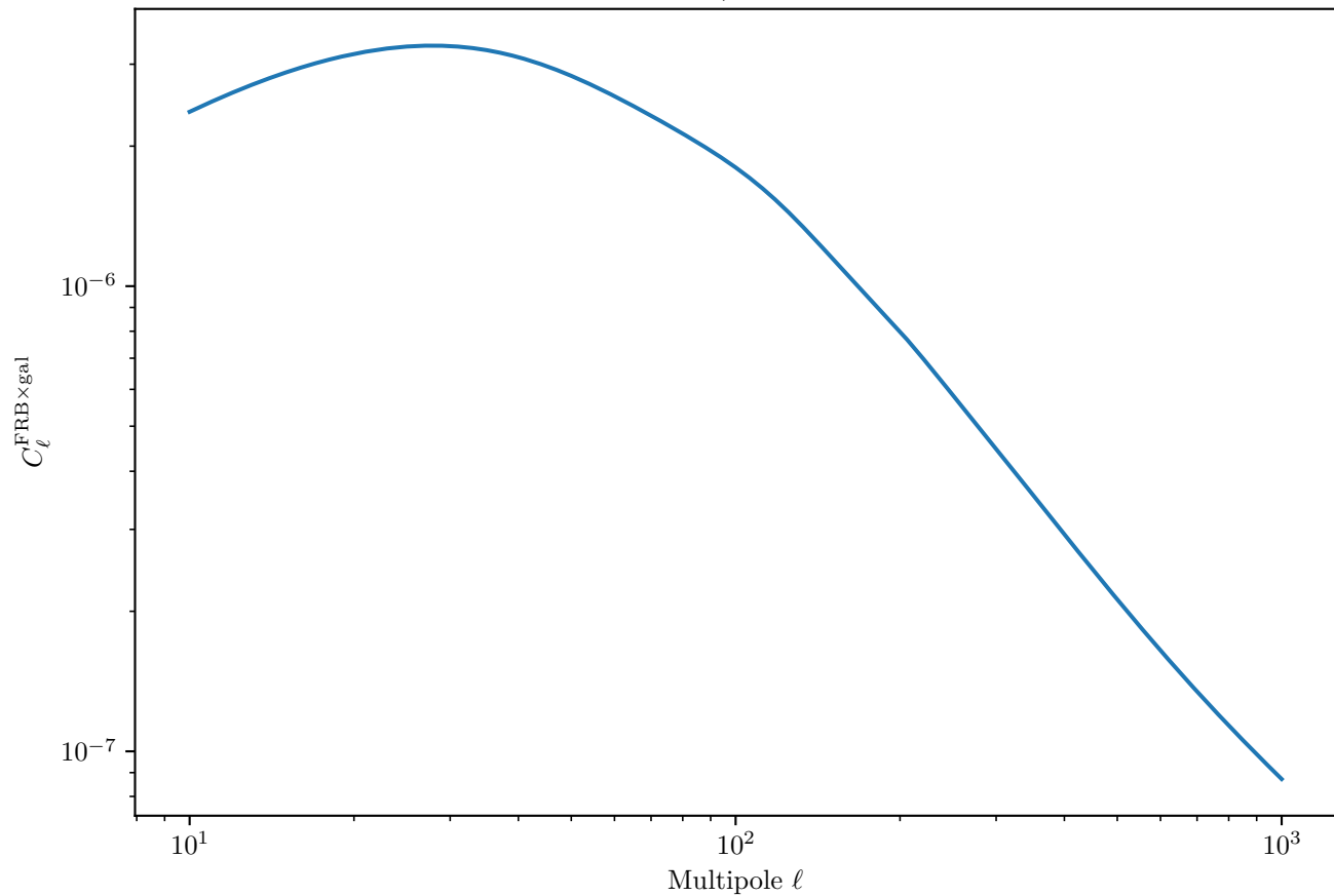
LSST Y10 FRB×Galaxy Cross-Correlation (Neutron Stars, Shallow Survey, Galaxy Bin 4)
