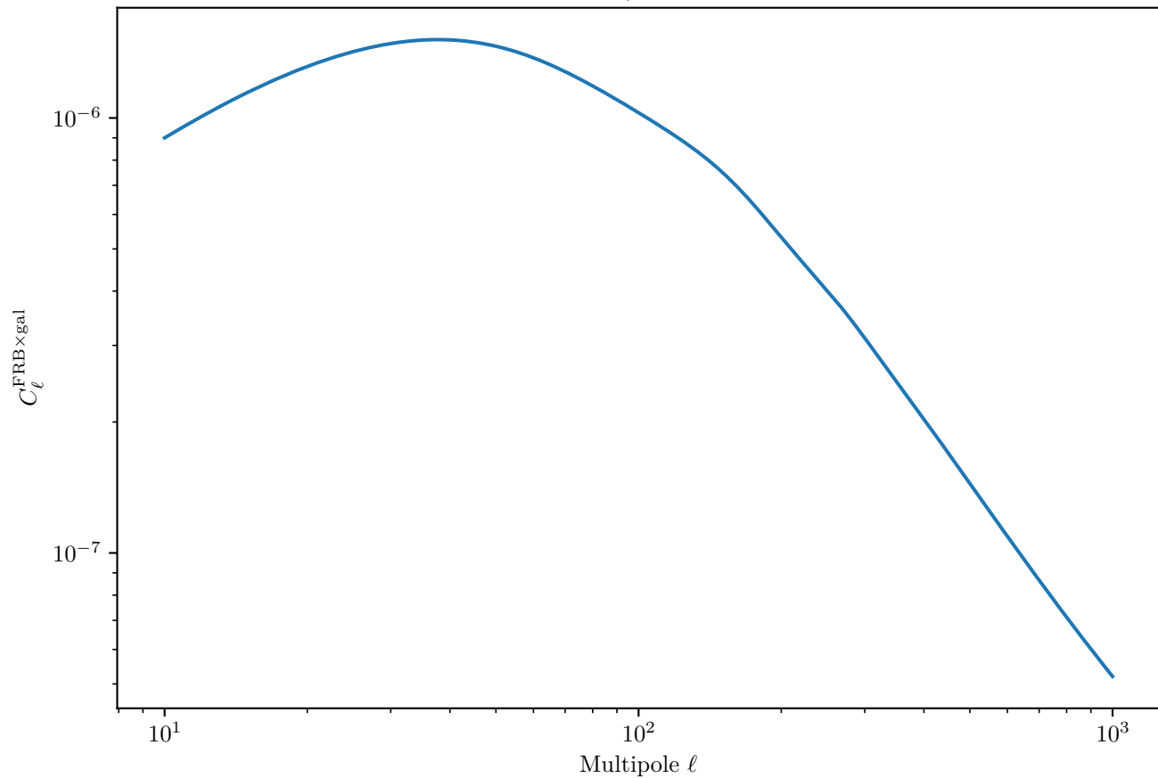
LSST Y10 FRB×Galaxy Cross-Correlation (Neutron Stars, Shallow Survey, Galaxy Bin 6)
