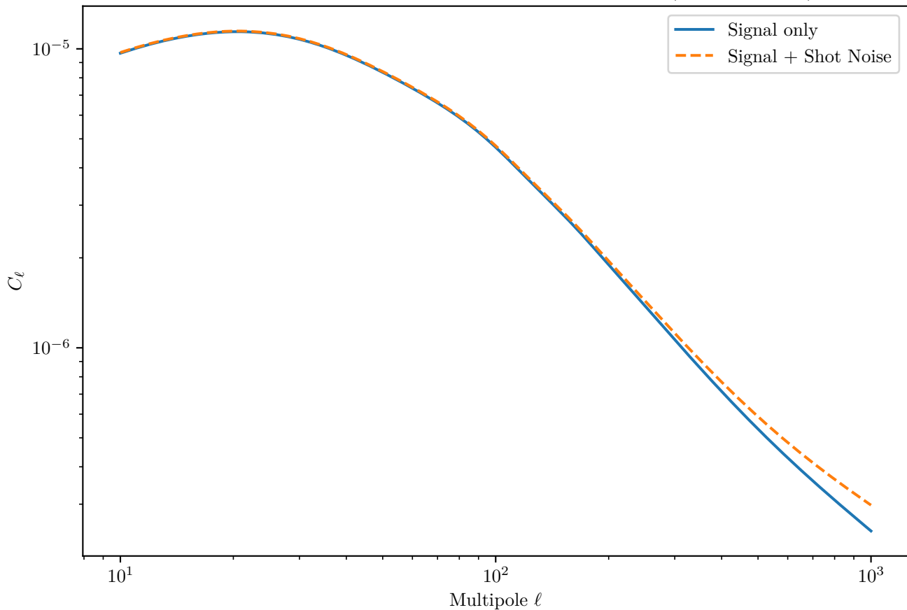
Galaxy Auto-Correlation Angular Power Spectrum (Bin 2 x Bin 2)
