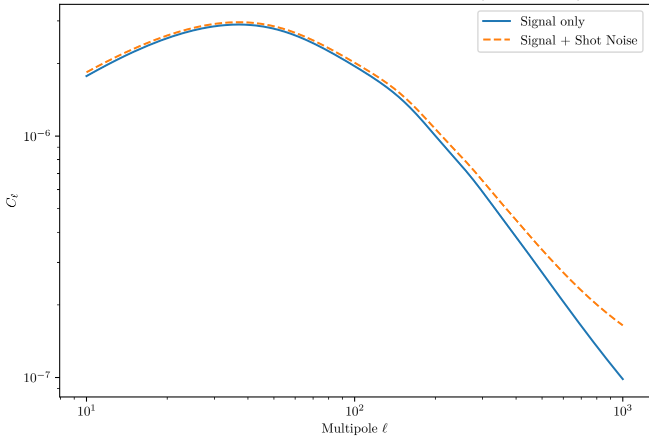
Galaxy Auto-Correlation Angular Power Spectrum (Bin 5 x Bin 5)
