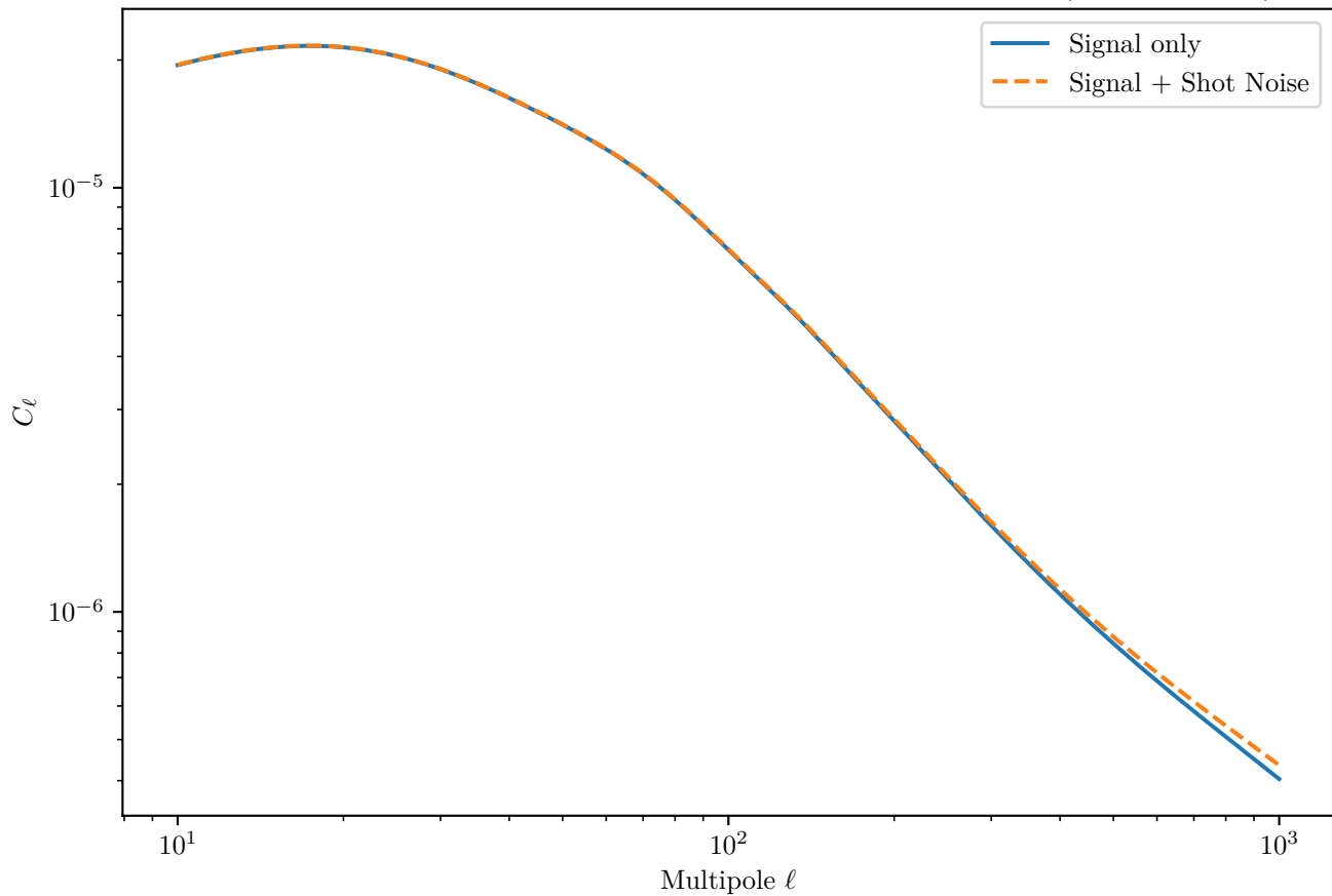
LSST Y10 Galaxy Auto-Correlation Angular Power Spectrum (Bin 2 x Bin 2)
