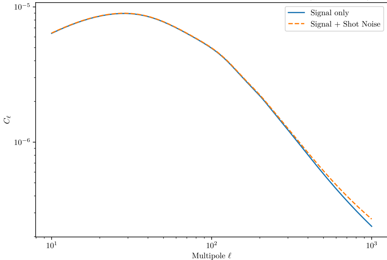
LSST Y10 Galaxy Auto-Correlation Angular Power Spectrum (Bin 4 x Bin 4)
