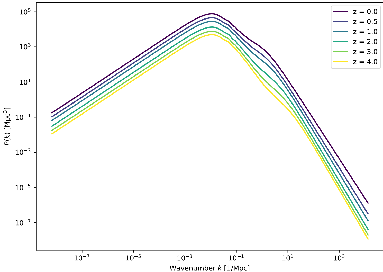
Nonlinear Matter Power Spectrum P(k, z) — Redshift Evolution
