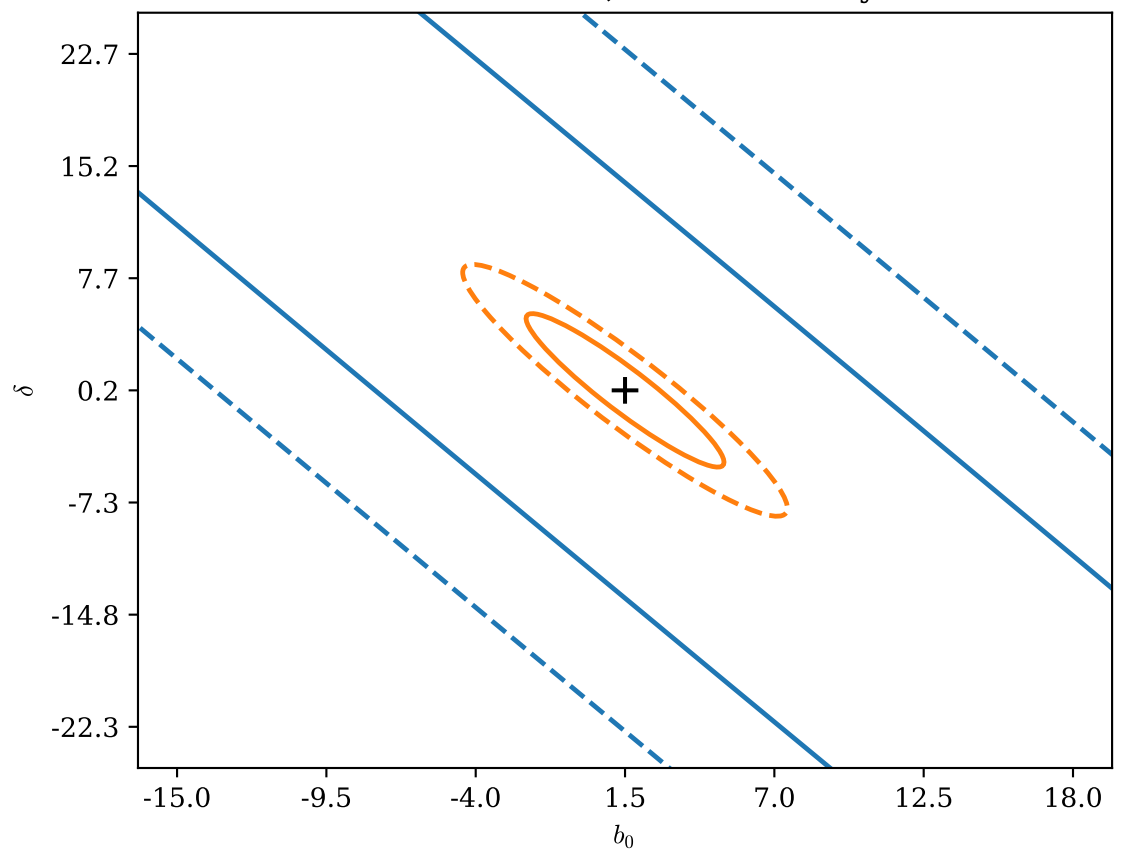
Neutron Stars, Shallow Survey
