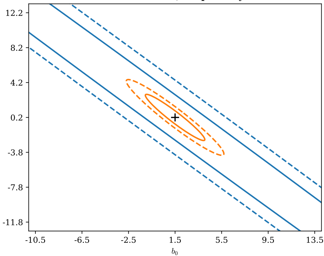
Neutron Stars, Deep Survey
