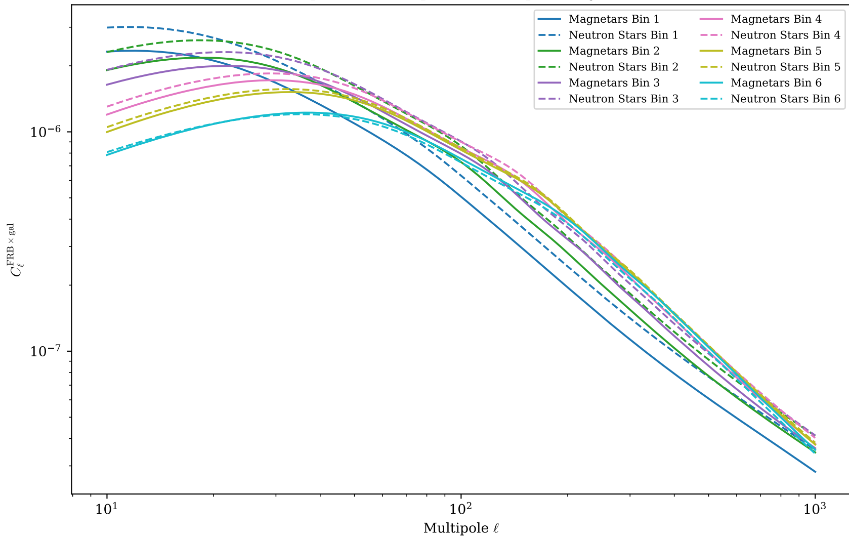
FRB Population Comparison (Deep Survey, all bins)
