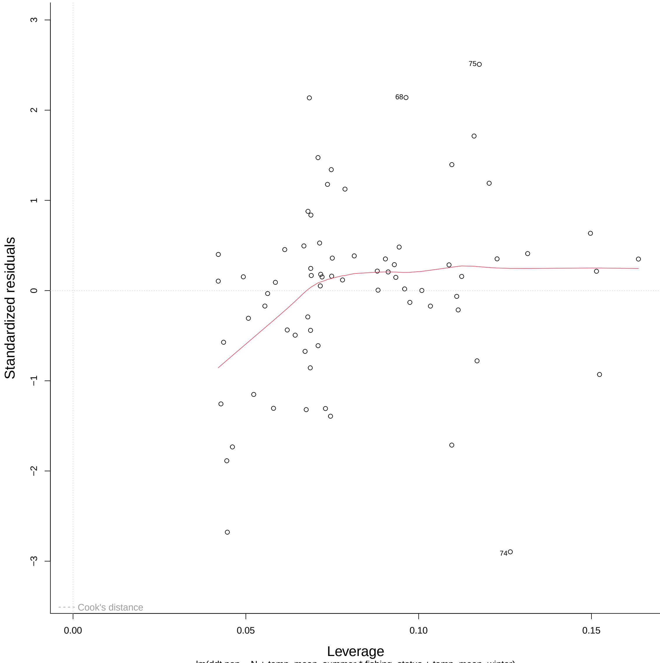
Residuals vs Leverage
