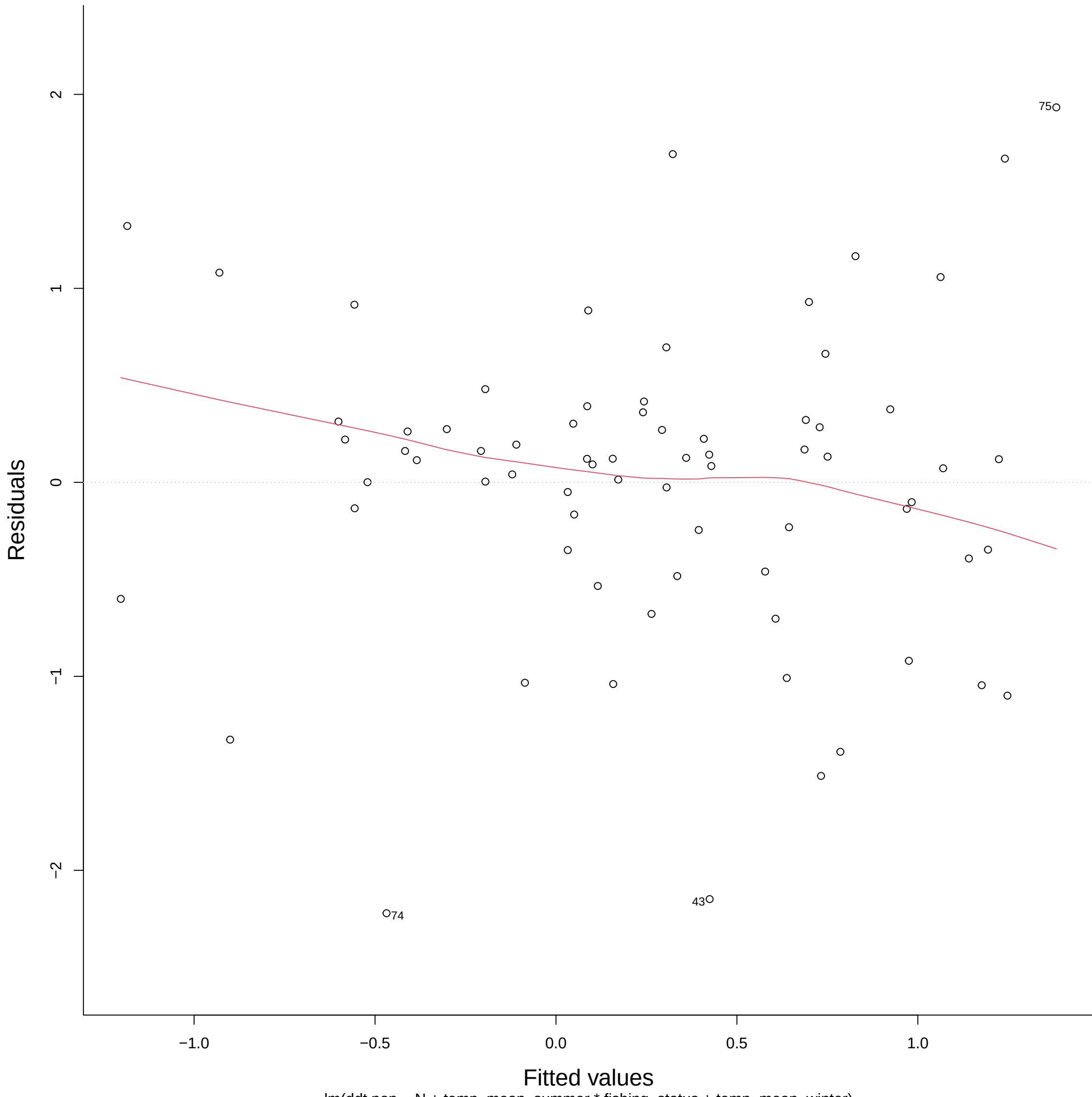
Residuals vs Fitted
