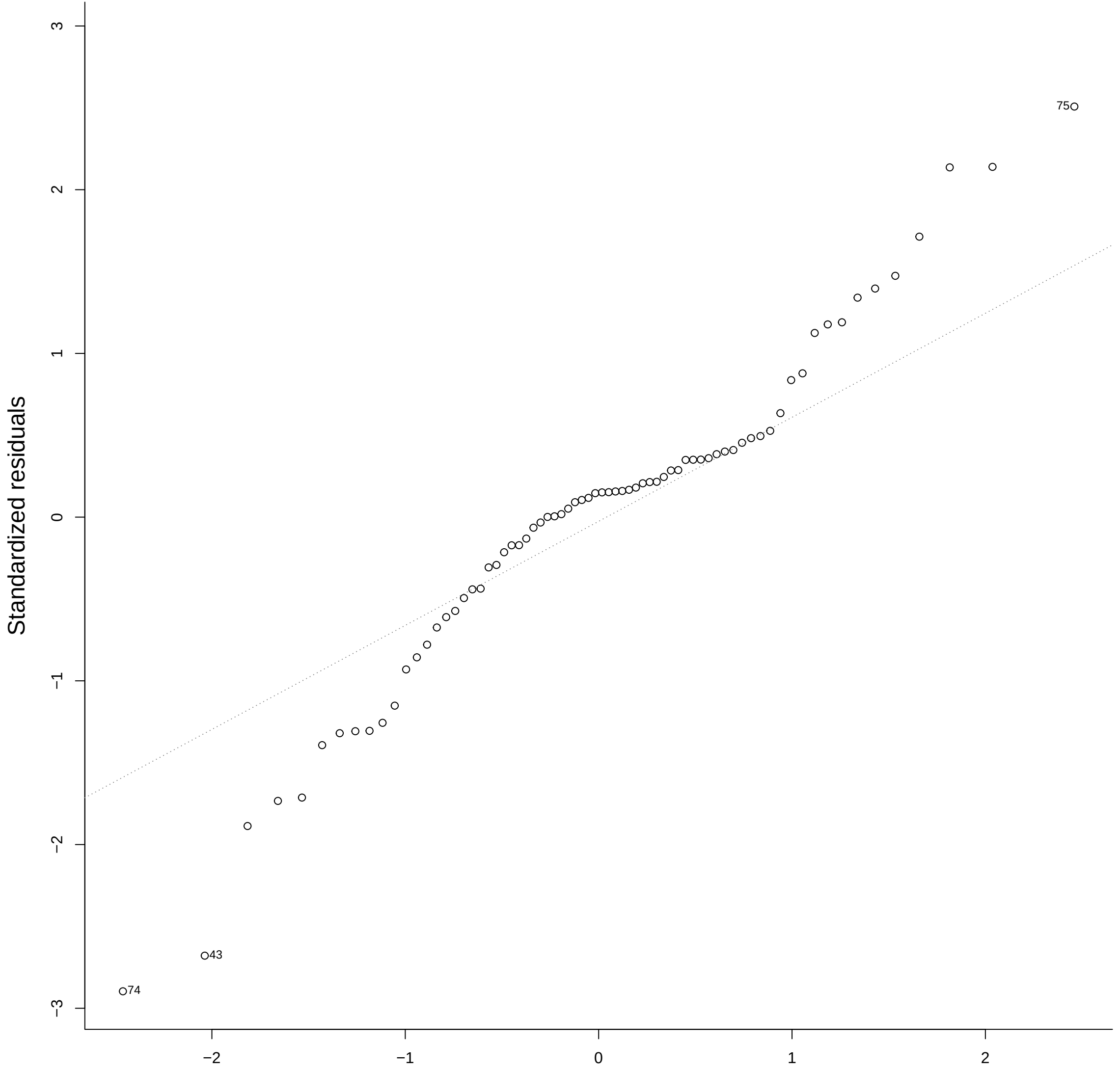
Q-Q Residuals
