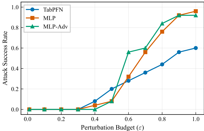
Dataset 1: FGSM Attack
