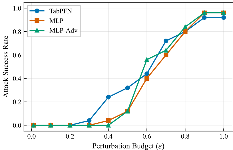
Dataset 1: PGD Attack
