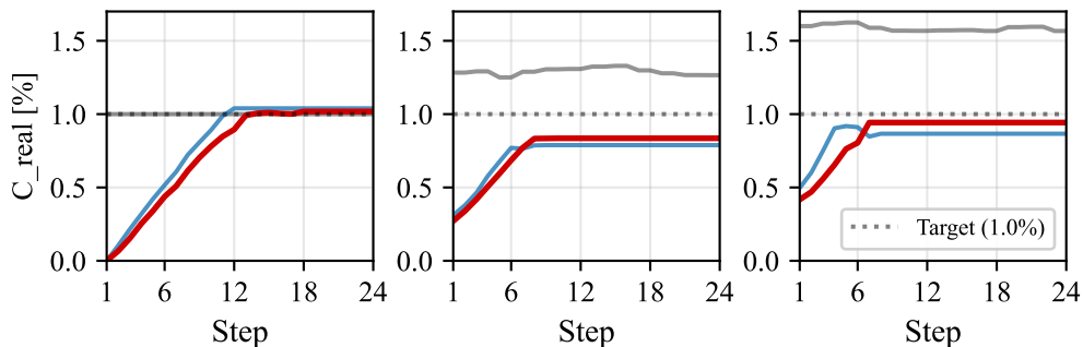
(c) Salinity Concentration - Step
