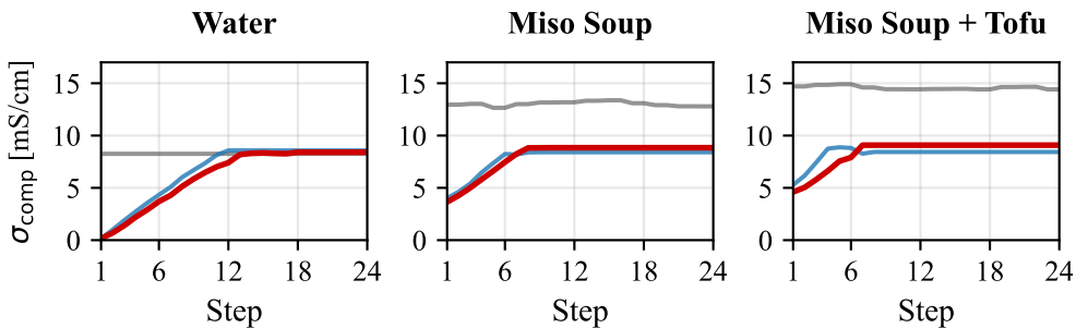
(a) Measured Conductivity (Compensated by Temperature) - Step
