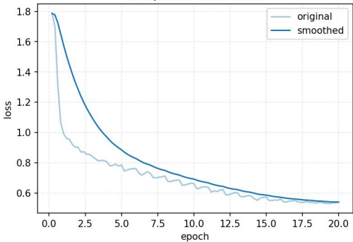
DeepseekMath-7B lora
