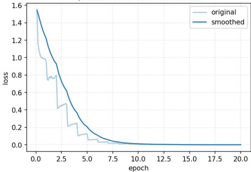
Qwen2.5-Math-1.5B-Instruct full
