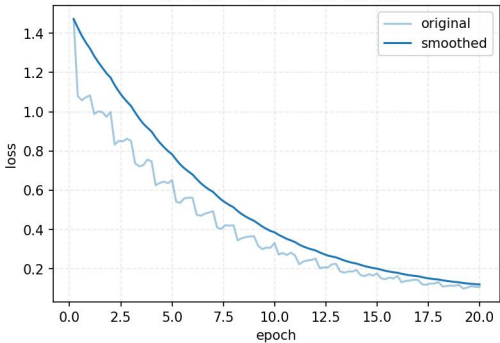
Qwen2.5-Math-7B-Instruct full
