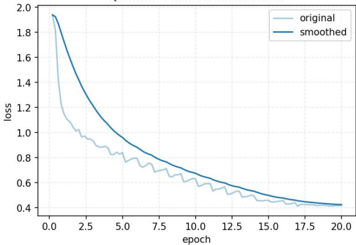
Qwen2.5-Math-7B-Instruct lora
