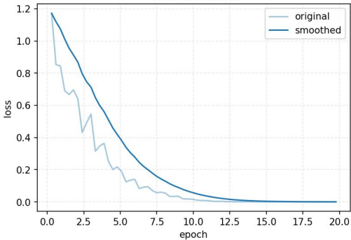
Mimo-7B-RL full
