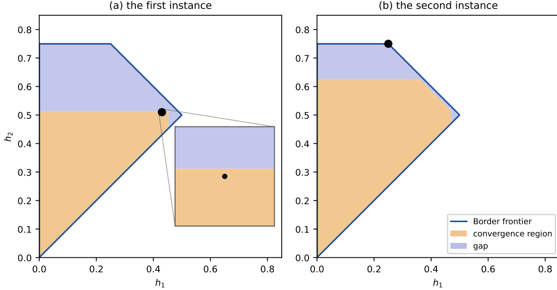
Figure 2: The pinned values of the two instances in (h_1, h_2) space at p = 1/2 , each panel drawn at its own (\tilde{h}_1, \tilde{h}_2) , geometry as in Figure 1. Panel (a), the first instance's pinned values lie inside the convergence region and against its boundary. Panel (b), the second's lie at the corner of the Border frontier, where both binding inequalities hold with equality. Both panels impose the model's ordering restriction h_1 < h_2 , so the sets shown are the Border set and the convergence region within the admissible wedge.
