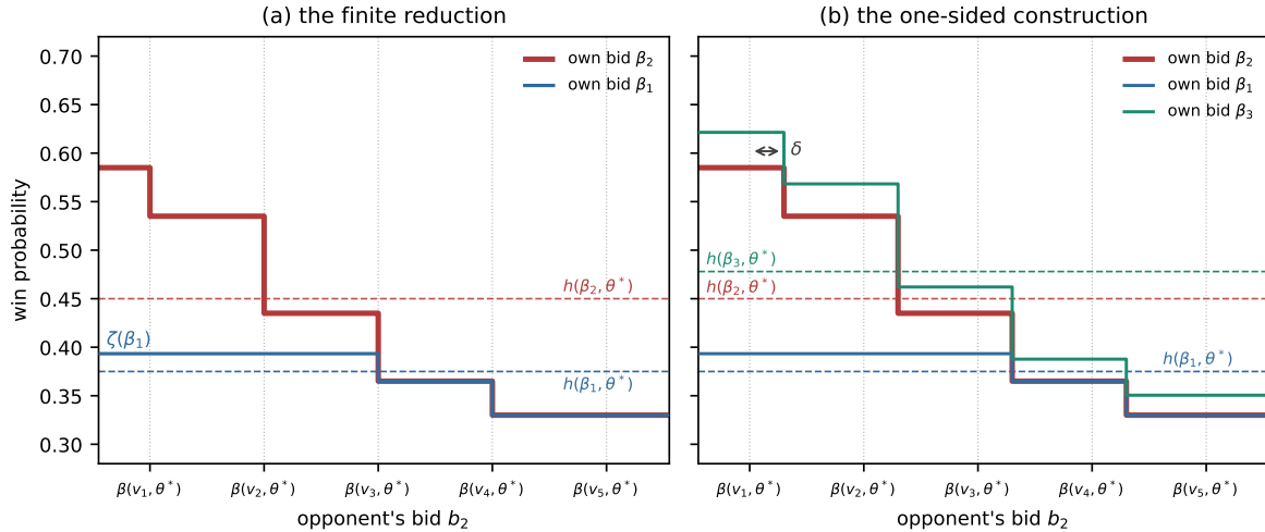
Figure 7: The constructions of Lemmas 9 and 10 at an illustrative five-value example with uniform type probabilities. Throughout, \beta_2 denotes the grid bid \beta(v_4, \theta^*) , \beta_1 an own-bid in (\beta(v_3, \theta^*), \beta_2) , and \beta_3 an own-bid in the window (\beta_2, \beta_2 + \delta) . Panel (a), cross-sections in the opponent's bid at own-bids \beta_2 and \beta_1 under the extension of Lemma 9. The mechanism is constant in the opponent's bid between grid bids by (CE)_0 , and at \beta_1 the win probabilities inherited from \beta_2 are capped at \zeta(\beta_1) by (TS), flat up to a threshold and following the inherited values beyond it. Dashed lines mark the level each cross-section averages to across the opponent's grid bids at \theta^* . Panel (b), the same cross-sections under the construction of Lemma 10 at shift \delta , the step boundaries moved upward by \delta by (CE)_\delta , together with the cross-section at \beta_3 , the \beta_2 values rescaled by h(\beta_3, \theta^*)/h(\beta_2, \theta^*) by (PS).
