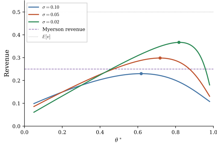
Figure 6: Revenue as a function of \theta^* in the correlated reserve price model with \psi(v, \theta) = v\theta and v \sim \text{Uniform}[0, 1] . Each curve corresponds to a different noise level \sigma . Dots indicate the revenue-maximising \theta^* . The dashed line marks Myerson's optimal auction revenue; the dotted line marks \mathbb{E}[v] = 1/2 .
