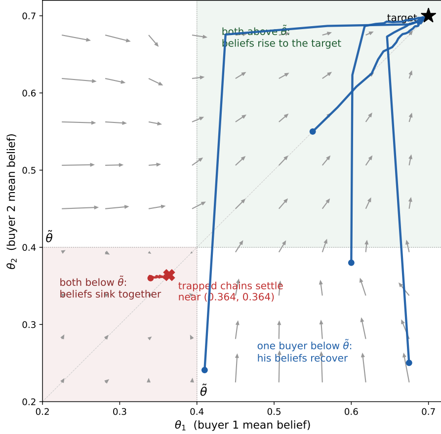
Figure 5: The second instance in the plane of the two buyers' mean beliefs. Each arrow is the simulated change in the two mean beliefs over 150 periods from priors concentrated at its base, averaged over 24 seed pairs, with length scaled by the square root of the displacement. The five paths are seed-mean trajectories over 60,000 periods from the marked starts, eight seed pairs each. Dotted lines mark the overlap belief \tilde{\theta} on each axis. Beliefs reach the target from every start with at least one belief above \tilde{\theta} and settle near (0.364, 0.364) from the start with both below it.
