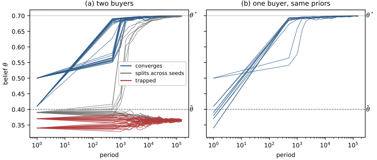
Figure 4: The same six priors under two buyers and under one. Panel (a), the two-buyer runs divide into three fates, and those starting below the overlap belief \tilde{\theta} stay below it. Panel (b), the single buyer converges from all six. Time is on a logarithmic scale. Panel (a) carries eight seeds per prior and panel (b) two. Converging chains settle at 0.6990 rather than exactly at \theta^* , which is the finite horizon and the posterior's residual spread and is common to both.
