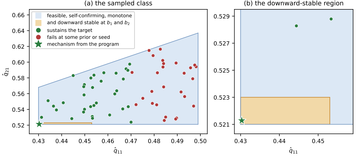
Figure 3: Mechanisms drawn from the class at the first instance, where the program of Proposition 4 is strictly feasible, sorted by simulated outcome. Blue shading is the sampled polytope of strictly feasible, self-confirming, monotone grid mechanisms. Amber is the part of it that also generates corrective feedback at both bids. Points are the sixty draws, coloured by simulated outcome at 125,000 periods, with the constructed mechanism starred. Panel (b) magnifies the amber region, which is some 0.023 wide and 0.002 tall.
