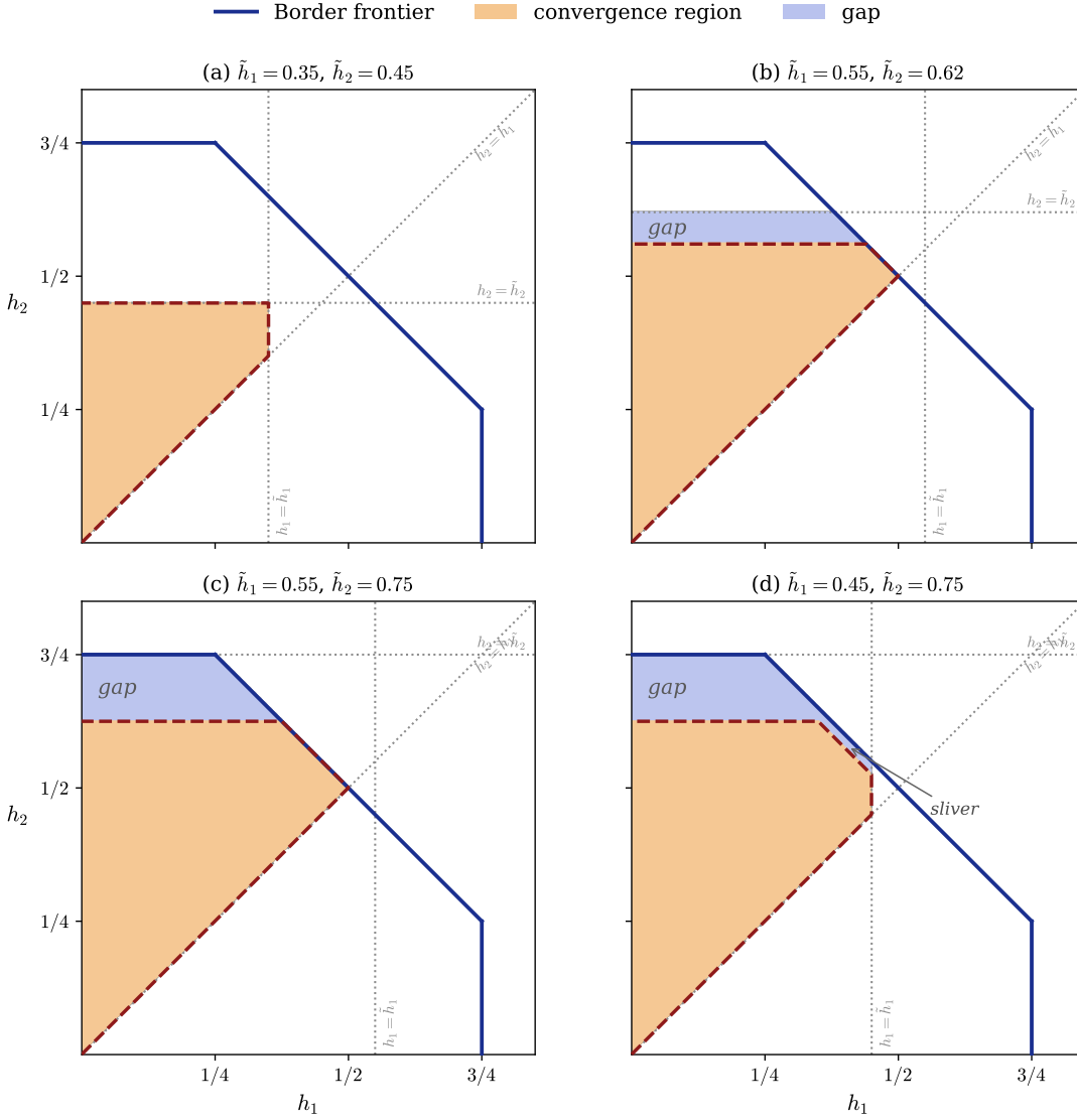
Figure 1: Border region vs. convergence region in (h_1, h_2) space for p = 0.5 , with (\tilde{h}_1, \tilde{h}_2) varying by panel. Shading is restricted to admissible pairs (h_1 < h_2, h_i < \tilde{h}_i) , so the Border region is the union of the convergence region and the gap. The regions coincide in panel (a), the band is widest in panel (c), and the sliver of panel (d) reflects the cap at b_1 .
