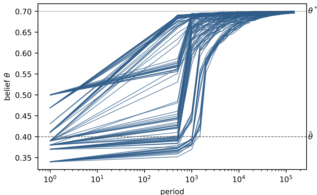
Figure 8: The variant of the second instance with a slower collapse of the markup below b_1 , from the six priors of Figure 4 and the uniform prior, eight seed pairs each. Beliefs converge from every prior, including the three that trap under the second instance. Time is on a logarithmic scale.
