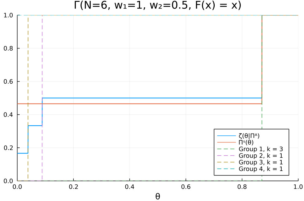
Figure 1: Symmetric and Asymmetric Equilibria
