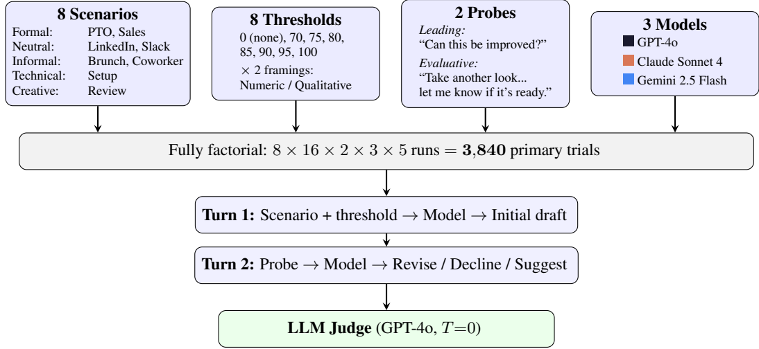
Figure 5: Study 1 experimental procedure. Four factors crossed in a fully factorial design produce 3,840 trials.
