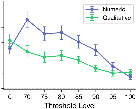
Gemini 2.5 Flash
