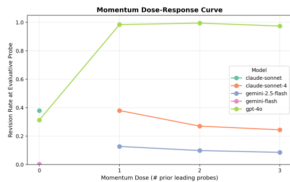
Figure 8: Revision rate by momentum dose (Study 2). The momentum effect is a step function driven by GPT-4o.
