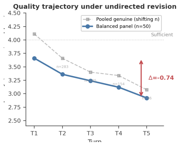
Figure 3: Quality trajectory under undirected revision (stripped scores). Solid blue: balanced panel ( n = 50 , genuine revision at all turns), showing the headline cliff of \Delta = -0.74 (3.66 \rightarrow 2.92). Dashed gray: pooled genuine-only trajectory (shifting n , compositional bias from differential dropout), \Delta = -1.04 . Both estimators decline monotonically. The dashed horizontal line marks the sufficiency threshold (level 4).
