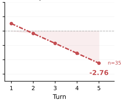
Qwen 3 235B
