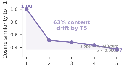
Semantic drift from original
