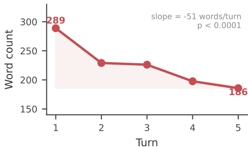
Responses shrink each turn
