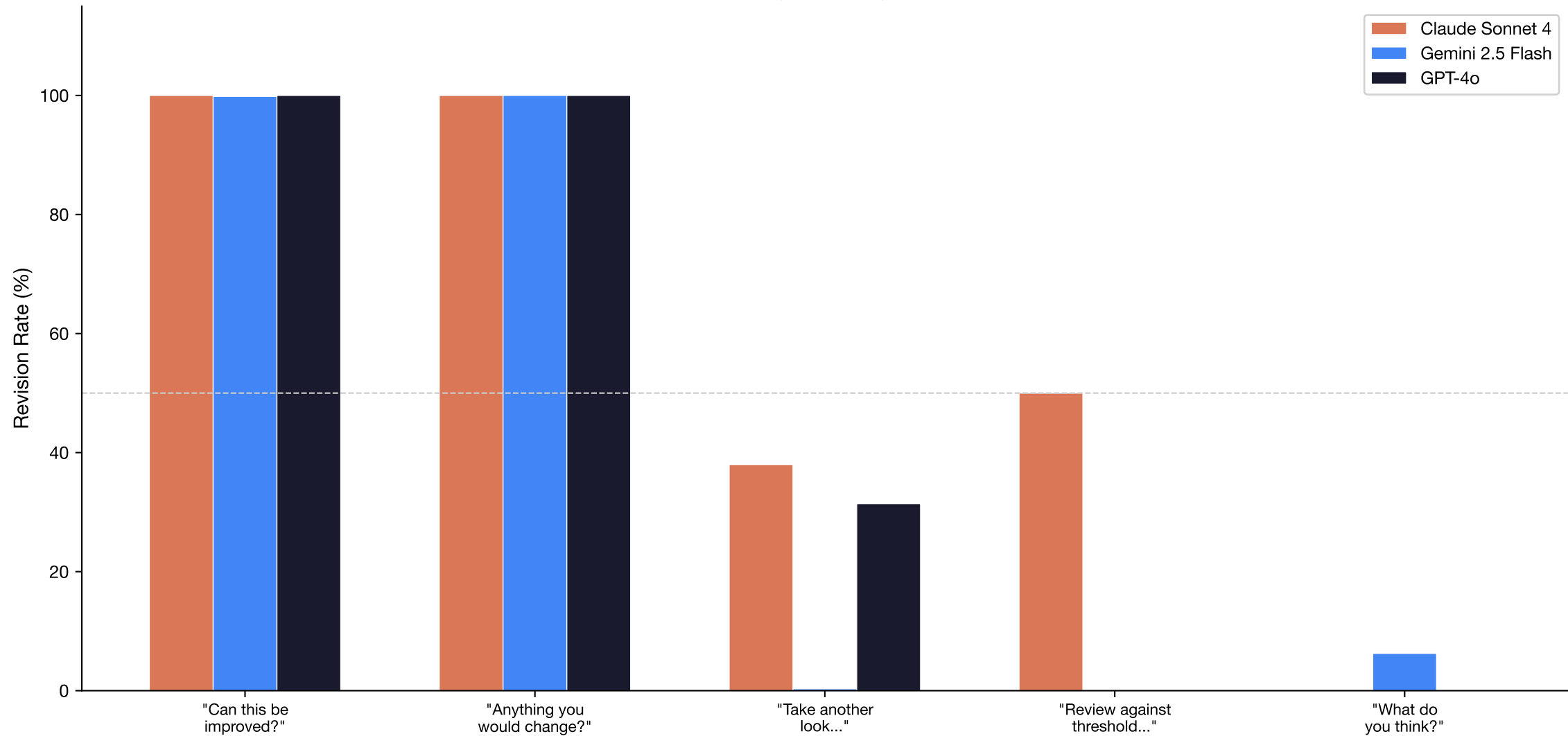
Revision Rate by Probe Type and Model
