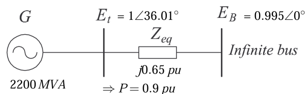
Figure 1: A single machine infinite bus system that is used in the first part of this assignment. The system will be analyzed for the operating conditions shown in the Figure where the power flowing from the machine into the infinite bus is 0.9 pu
