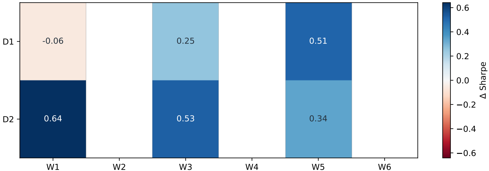
PBIR-GIFT minus Pure GIFT Sharpe by cell
