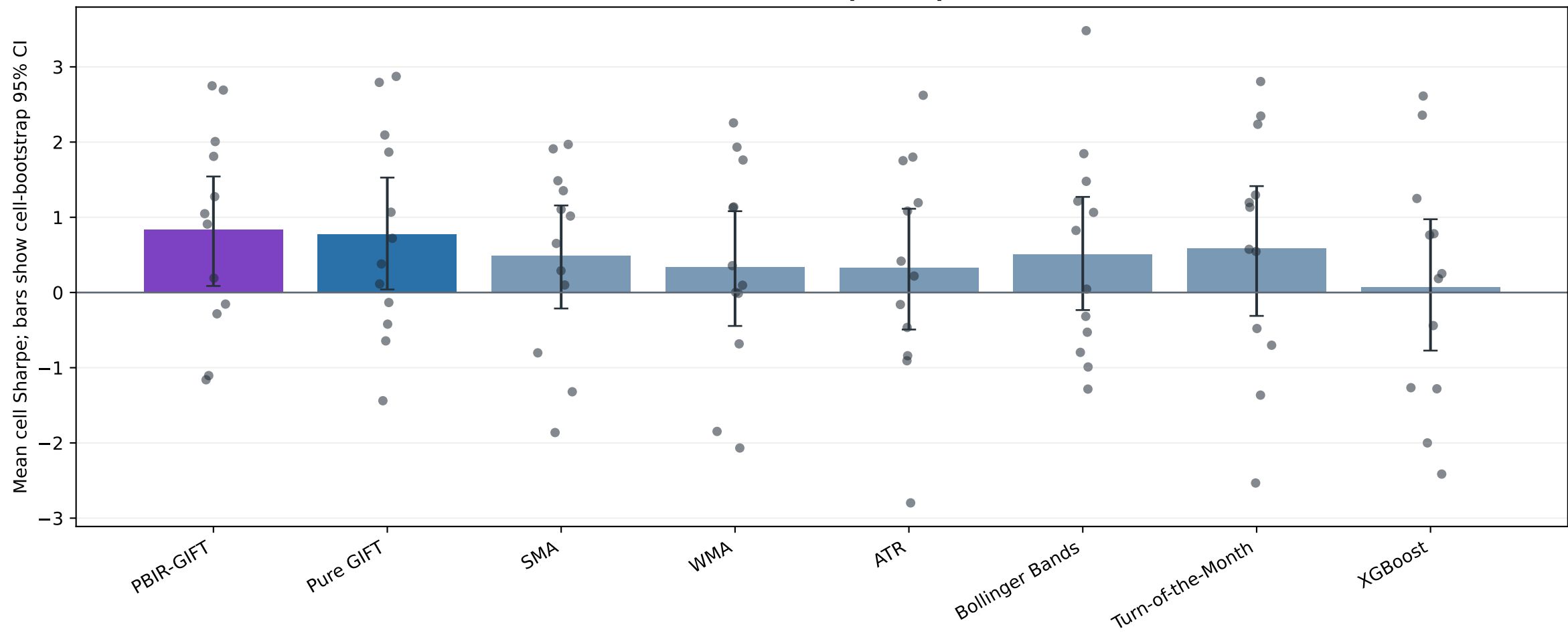
Cross-window Sharpe comparison
