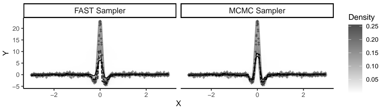
Heart Beat Relationship (n=500)
