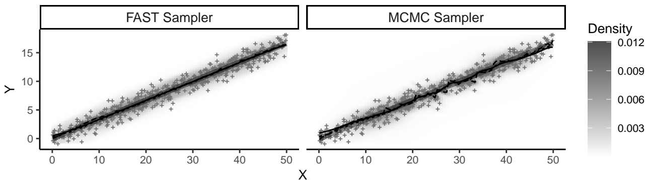
Nonlinear Relationship (n=500)
