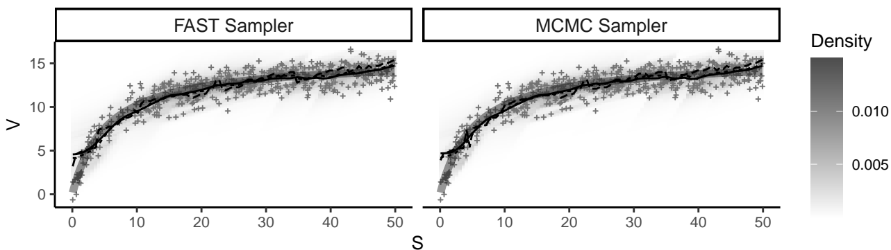
Polynomial Relationship (n=500)
