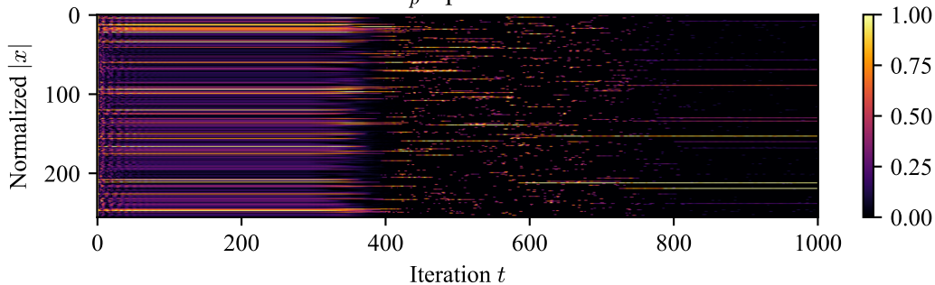
\ell_p Squeeze
