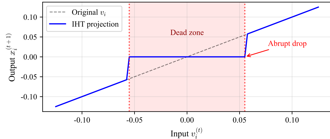
(a) IHT: Hard Thresholding
