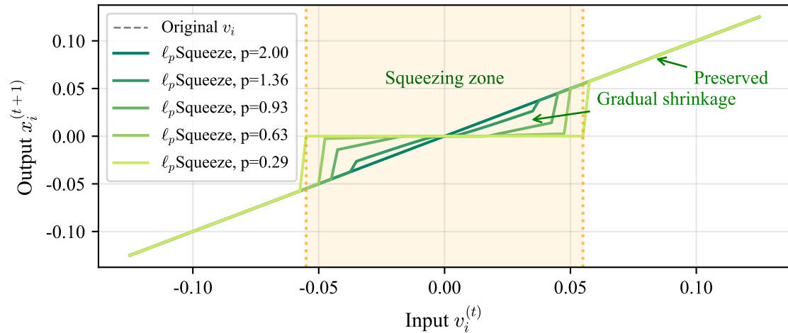
(b) \ell_p Squeeze: Progressive Squeezing
