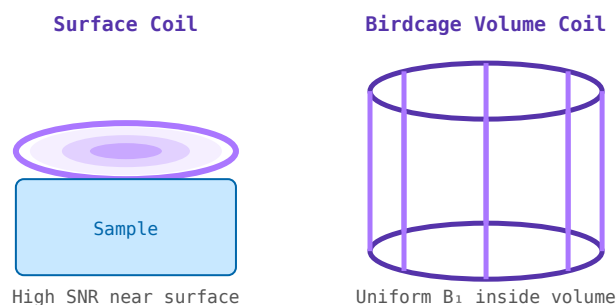
Figure 82.2: Left: surface coil — high local SNR, non-uniform. Right: birdcage volume coil — uniform B_1 throughout volume.
