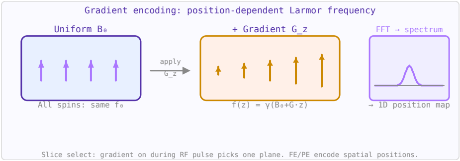
Figure 77.1: Gradient fields make Larmor frequency position-dependent. FFT of the NMR signal then maps frequencies to spatial positions.
