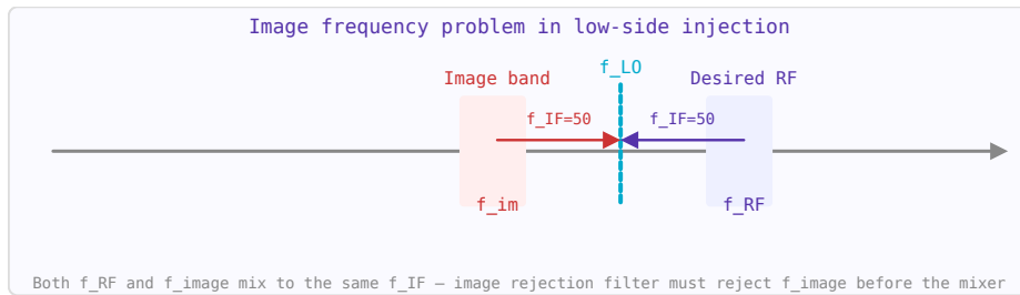
Figure 59.2: The image frequency f_{image} = f_{LO} - f_{IF} (low-side injection) produces the same IF as the desired signal.
