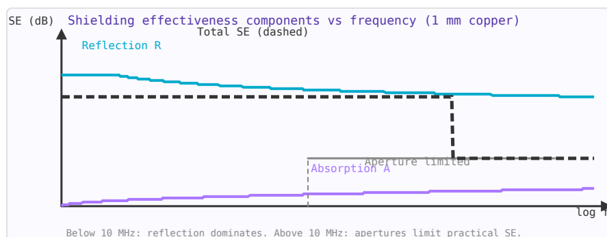
Figure 73.1: Shielding effectiveness components for 1 mm copper: reflection (blue), absorption (purple), and aperture limit (grey).
