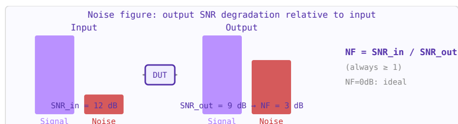
Figure 37.1: Noise figure quantifies how much a device degrades SNR. A 3 dB NF device adds as much noise as a matched resistor at 290 K.
