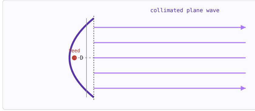
Figure 53.1: A parabolic reflector converts the spherical wave from a focal feed into a plane wave across the aperture, forming a narrow pencil beam.
