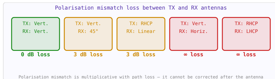
Figure 50.2: Polarisation mismatch loss for common antenna orientation combinations.
