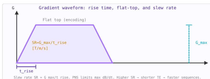
Figure 77.2: Trapezoidal gradient waveform. Rise time t_{\text{rise}} = G_{\text{max}}/SR limits shortest achievable echo time.
