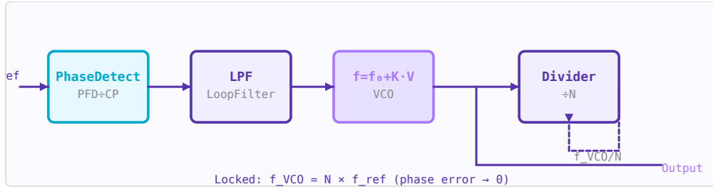
Figure 45.1: PLL block diagram: PFD compares f_{\text{ref}} to f_{\text{VCO}}/N ; loop filter drives VCO to lock frequency and phase.
