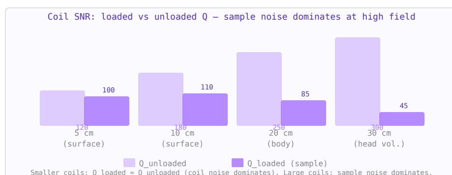
Figure 84.1: Loaded vs unloaded Q for MRI receive coils. When Q_{\text{loaded}} \ll Q_{\text{unloaded}} , sample noise dominates — the coil is in the "sample-noise dominated" regime where \text{SNR} \propto \omega_0 B_1 / \text{coil} .
