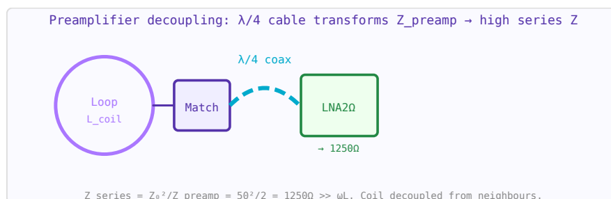
Figure 85.1: Preamplifier decoupling circuit. \lambda/4 cable transforms 2\Omega LNA input to 1250\Omega high series impedance in the coil loop.
