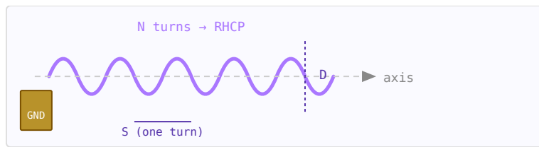
Figure 52.1: Axial-mode helix: N turns of diameter D , turn spacing S , fed against a ground plane.
