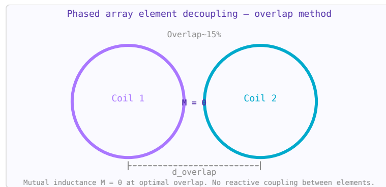
Figure 86.2: Overlapping coil decoupling: optimal overlap distance ( \approx 15\% of diameter) sets mutual inductance M = 0 .
