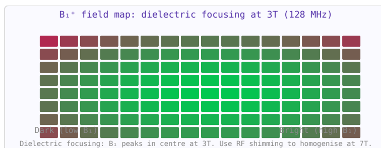
Figure 88.2: B_1^+ field map simulation at 3T. Constructive interference of RF waves creates a bright central spot in the phantom.
