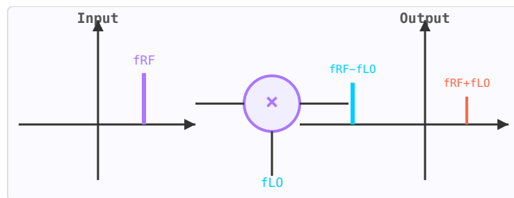
Figure 47.1: Mixer produces sum ( f_{RF} + f_{LO} , orange) and difference ( f_{RF} - f_{LO} , blue) frequency components.
