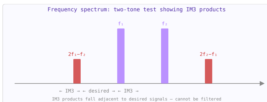
Figure 40.2: Two-tone test: input tones f_1 and f_2 (purple) generate IM3 products at 2f_1 - f_2 and 2f_2 - f_1 (red) close to the passband.
