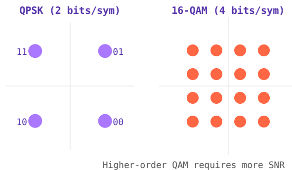
Figure 48.2: QPSK (4 symbols, 2 bits/sym) and 16-QAM (16 symbols, 4 bits/sym) constellation diagrams.
