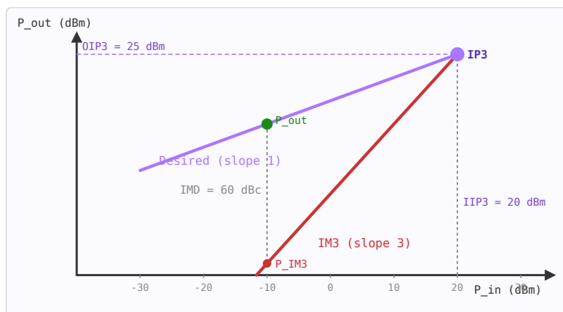
Figure 40.1: Output power vs input power. Signal: slope 1. IM3 products: slope 3. They extrapolate to the IP3 intercept point.
