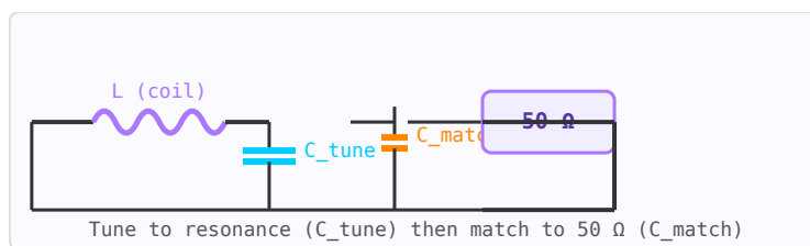
Figure 81.2: Coil tuning and matching circuit: C_{\text{tune}} resonates the coil at f_{\text{Larmor}} ; C_{\text{match}} transforms impedance to 50\ \Omega .
