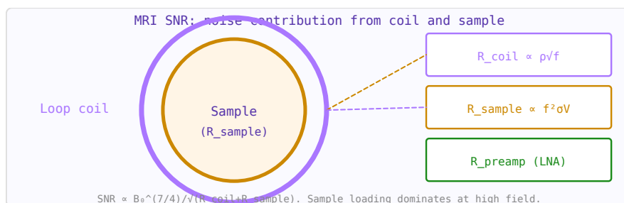
Figure 84.2: MRI coil SNR model: noise sources are coil resistance R_c , sample loading R_s , and preamplifier R_p .
