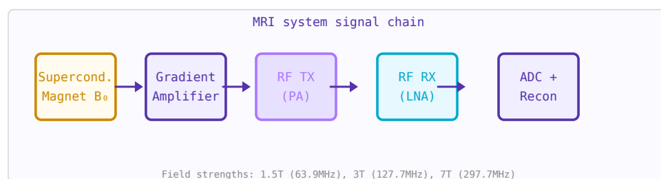
Figure 76.1: MRI system: superconducting magnet, gradient amplifiers, RF transmit power amp, LNA receiver, and digital reconstruction.
