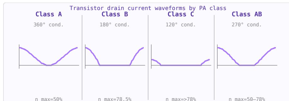
Figure 38.1: Drain current waveforms by amplifier class. Less conduction → higher efficiency but more distortion.
