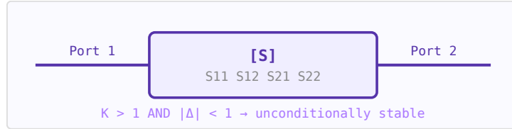
Figure 34.1: Two-port device described by S-parameters. Stability is assessed from S11, S12, S21, S22 alone.
