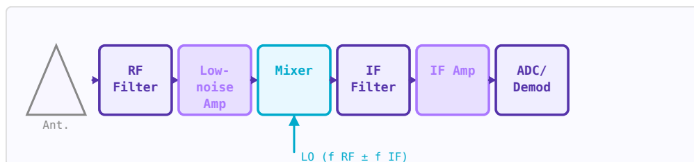
Figure 59.1: Superheterodyne receiver signal flow. The RF filter sets image rejection; the IF filter provides channel selectivity.
