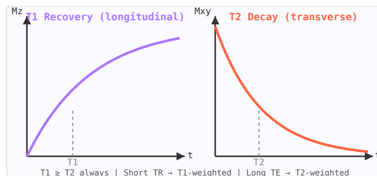
Figure 79.1: T_1 recovery (purple) and T_2 decay (orange) curves. T_1 \geq T_2 always. Different tissues have different values.
