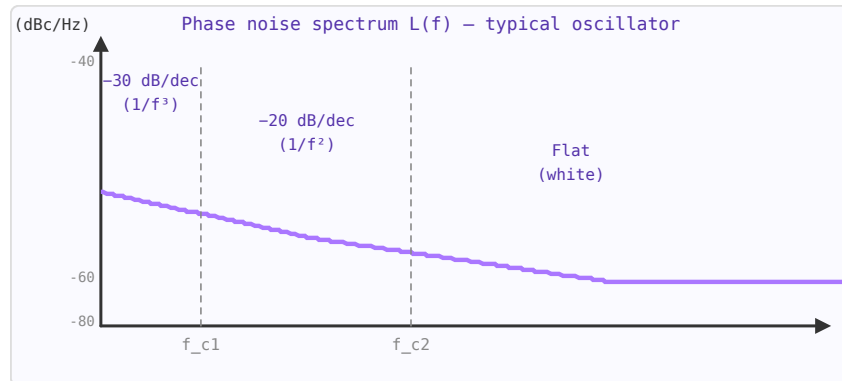
Figure 44.1: Phase noise L(f) showing three regions: 1/f^3 (flicker FM), 1/f^2 (white FM / Leeson), and flat (white phase noise floor).
