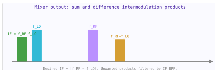
Figure 47.2: Mixing products: desired IF (green), input tones (blue/purple), and upper sideband (orange).
