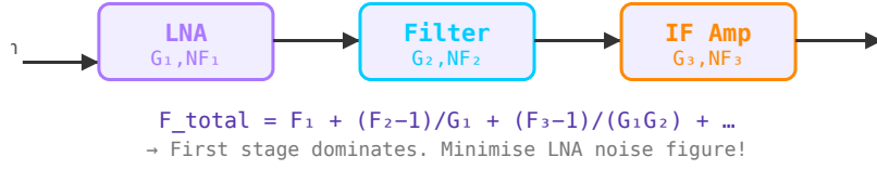
Figure 37.2: Cascaded receiver chain. LNA noise figure dominates because later stages are divided by preceding gains.
