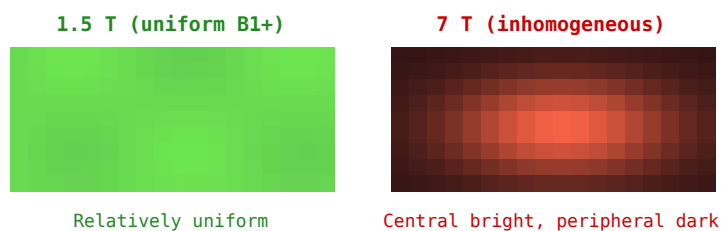
Figure 89.2: B_1^+ field maps at 1.5 T (uniform, left) and 7 T (inhomogeneous, right), illustrating how wavelength effects create SAR hotspots at high field.
