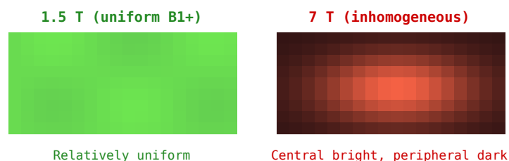
Figure 88.1: Simulated B_1^+ maps: 1.5 T (left, uniform) vs 7 T (right, central brightening due to constructive EM interference).
