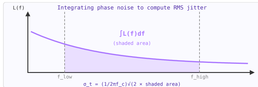
Figure 44.2: RMS jitter equals the square root of twice the integrated phase noise (linear) over the specified bandwidth.
