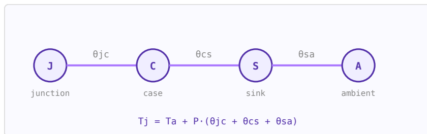
Figure 39.1: The junction-to-ambient thermal chain: die \rightarrow case \rightarrow heat sink \rightarrow air, each stage a thermal resistance in ^{\circ}\text{C}/\text{W} .
