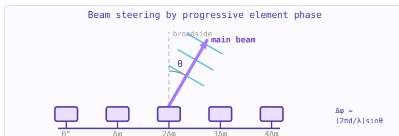
Figure 86.1: Phased array uses progressive phase shifts (implemented by phase shifters) to steer the main beam electronically.
