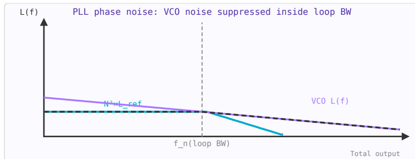
Figure 45.2: PLL output phase noise: inside loop BW = reference noise \times N^2 . Outside = free-running VCO noise. Total = worst of the two.
