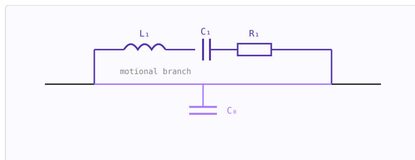
Figure 42.1: Butterworth–Van Dyke model: motional L_1 – C_1 – R_1 (the mechanical resonance) shunted by the static holder capacitance C_0 .
