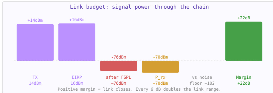
Figure 66.1: Link budget bar chart: TX power flows through gains and losses. Green margin bar = working link.
