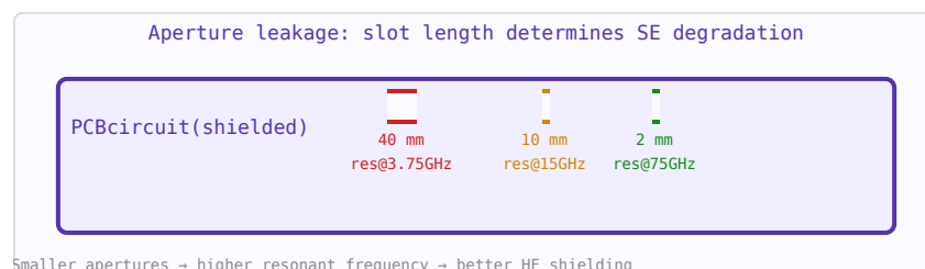
Figure 73.2: Aperture resonant frequency = c/(2L) . Smaller holes give better HF shielding at the cost of airflow.
