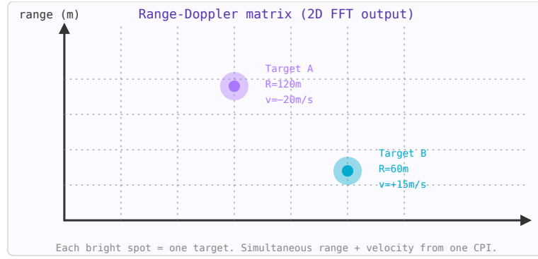
Figure 68.2: Range-Doppler matrix from 2D FFT. Range (vertical axis) and velocity (horizontal) resolved simultaneously.
