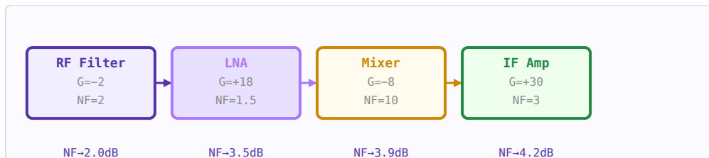
Figure 61.1: Cumulative noise figure stabilises after the LNA. First stage and its gain dominate the system NF.
