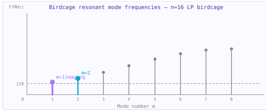
Figure 83.2: Birdcage resonant mode frequencies vs mode number m . Mode m=1 is the imaging mode (uniform field). Higher modes are spurious.
