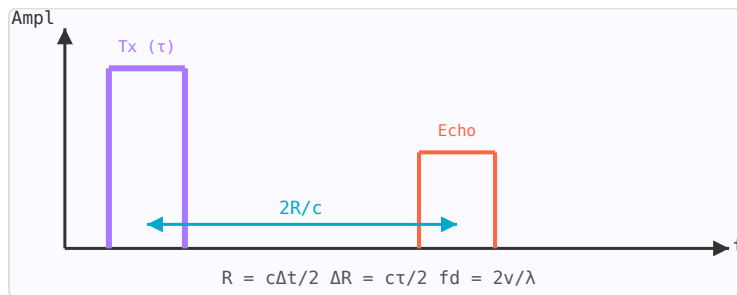
Figure 67.1: Radar timing diagram: transmit pulse (purple, width \tau ) and echo (orange). Range R = c\Delta t/2 ; resolution \Delta R = c\tau/2 .
