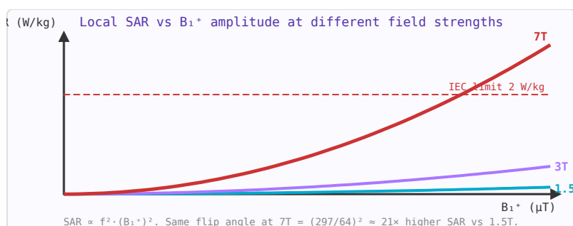
Figure 89.1: Local SAR grows with B_1^+ squared and with frequency squared. Managing SAR is the key challenge at ultra-high field (7T+).
