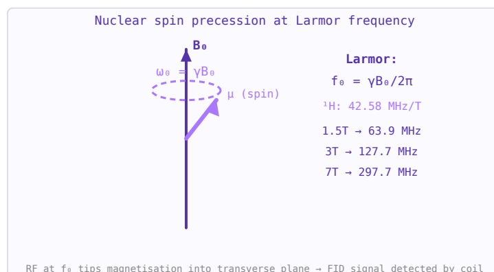
Figure 75.1: Larmor precession: spin \mu precesses around B_0 at \omega_0 = \gamma B_0 . RF excitation at this resonance frequency creates NMR signal.
