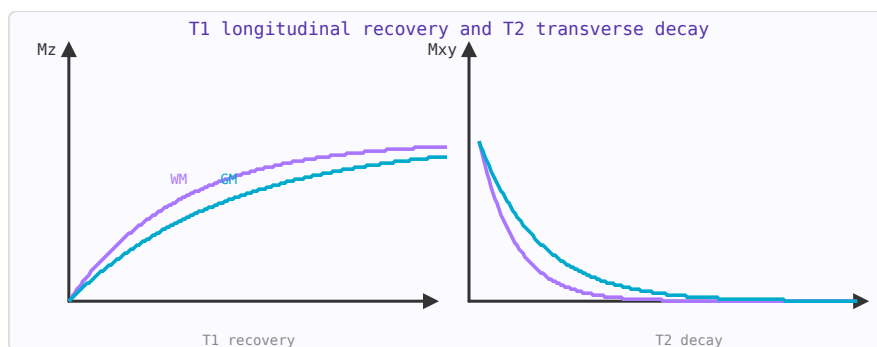
Figure 79.2: T1: longitudinal magnetisation recovers exponentially toward M_0 . T2: transverse magnetisation decays. Tissue contrast comes from T1/T2 differences.
