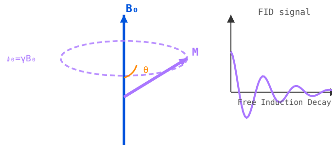
Figure 75.2: Left: M precessing around B_0 at \omega_0 = \gamma B_0 . Right: free induction decay (FID) signal after a 90^\circ pulse.
