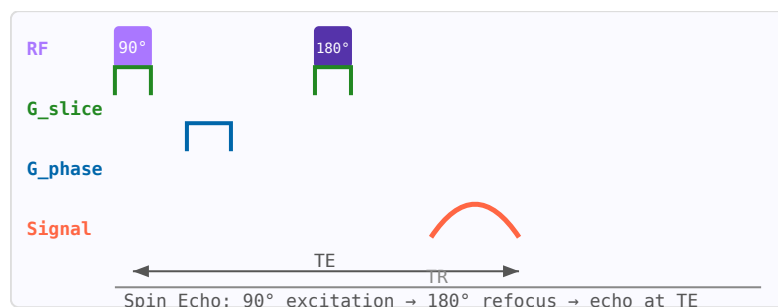
Figure 78.1: Spin echo pulse sequence: 90^\circ excitation, 180^\circ refocus at TE/2 , echo at TE . TR sets T1 weighting.
