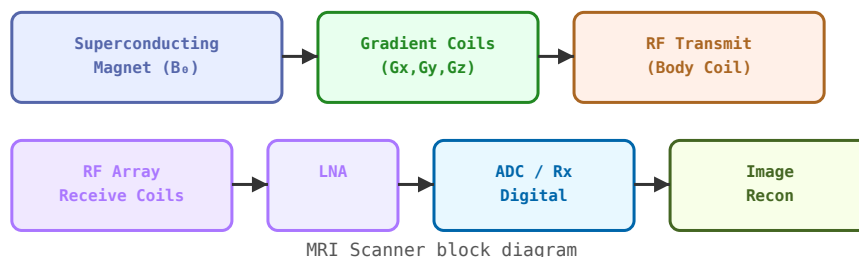
Figure 76.2: MRI scanner block diagram showing magnet, gradient coils, RF transmit/receive chains, and image reconstruction.
