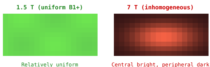
Figure 80.2: B_1^+ inhomogeneity: uniform at 1.5 T (left) but strong central brightening at 7 T (right) creating signal non-uniformity.
