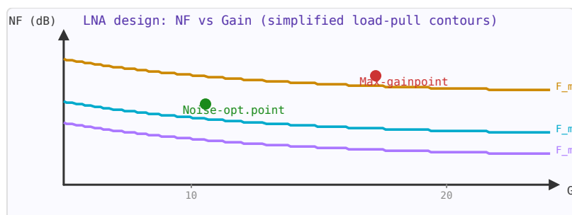
Figure 33.2: LNA tradeoff: minimum NF and maximum gain are different operating points. For first-stage LNA, prioritise NF.
