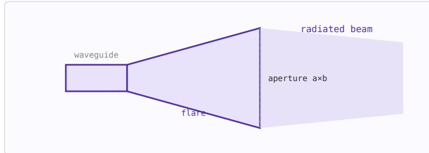
Figure 53.2: A pyramidal horn tapers the guide to a rectangular aperture a \times b ; a conical horn flares a circular guide to a diameter D .
