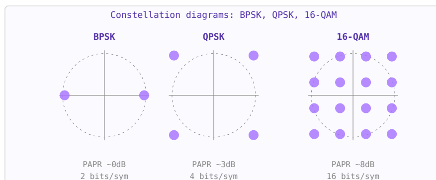
Figure 48.1: Constellation diagrams. More dots per unit area = higher spectral efficiency but requires better SNR.
