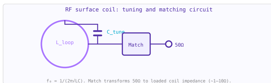
Figure 81.1: RF coil tuning: parallel capacitor C_{\text{tune}} resonates loop inductance L . Matching network presents 50 \Omega to the coaxial cable.
