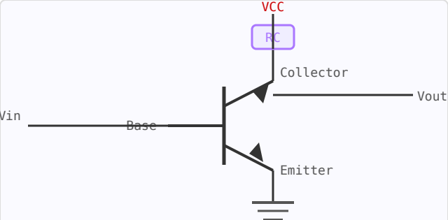
Common-Emitter (NPN BJT) Amplifier
