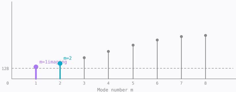
f (MHz) Birdcage resonant mode frequencies – n=16 LP birdcage
