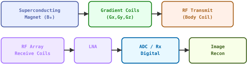
MRI Scanner block diagram
