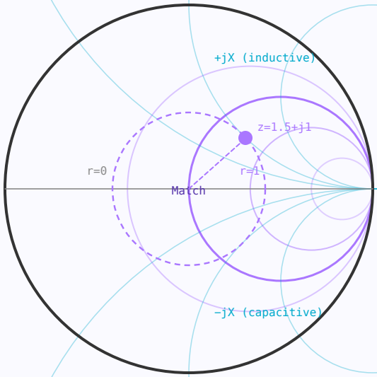
Annotated Smith Chart (normalised to Z_0 )
