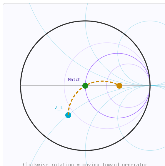
Figure 13.2: Smith Chart matching path: L_{load} (blue) \rightarrow \lambda/4 rotation (orange) \rightarrow matched (green).
