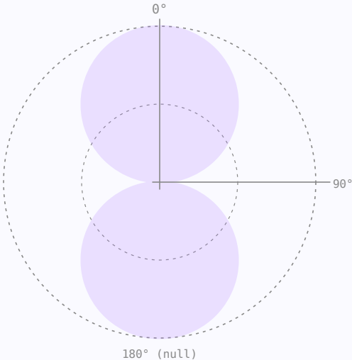
Half-wave dipole elevation pattern – figure-8 shape
