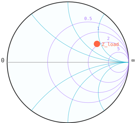
Smith Chart (normalised to Z_0 )
