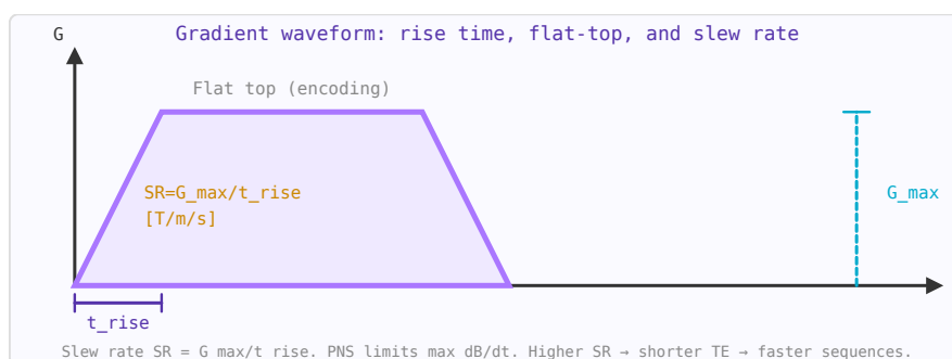
Figure 52.2: Trapezoidal gradient waveform. Rise time t_{\text{rise}} = G_{\text{max}}/SR limits shortest achievable echo time.
