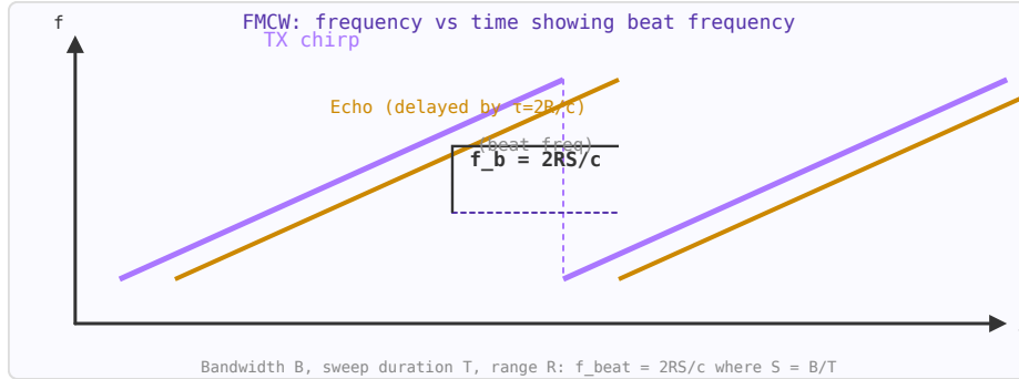
Figure 47.1: FMCW: TX sweeps from f_{\text{low}} to f_{\text{high}} ; echo arrives delayed by \tau=2R/c ; beat frequency f_b \propto range.
