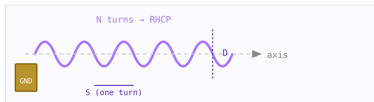
Figure 41.1: Axial-mode helix: N turns of diameter D , turn spacing S , fed against a ground plane.
