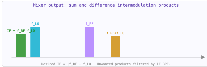
Figure 36.2: Mixing products: desired IF (green), input tones (blue/purple), and upper sideband (orange).
