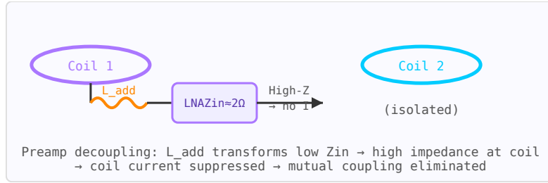
Figure 60.2: Preamplifier decoupling: L_{add} resonates with C_{match} , transforming the low preamp Z_{in} to high impedance at the coil loop, suppressing inter-coil coupling.
