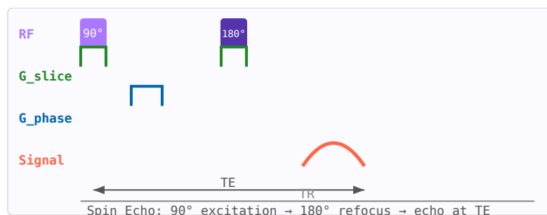
Figure 53.1: Spin echo pulse sequence: 90^\circ excitation, 180^\circ refocus at TE/2 , echo at TE . TR sets T1 weighting.
