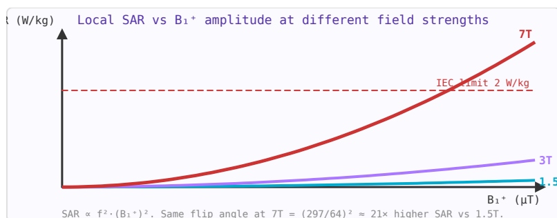
Figure 64.1: Local SAR grows with B_1^+ squared and with frequency squared. Managing SAR is the key challenge at ultra-high field (7T+).
