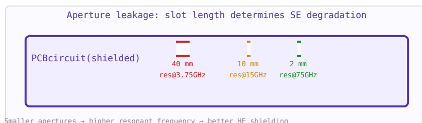
Figure 48.2: Aperture resonant frequency = c/(2L) . Smaller holes give better HF shielding at the cost of airflow.
