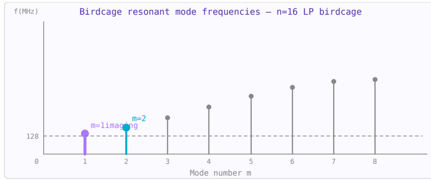
Figure 58.2: Birdcage resonant mode frequencies vs mode number m . Mode m=1 is the imaging mode (uniform field). Higher modes are spurious.
