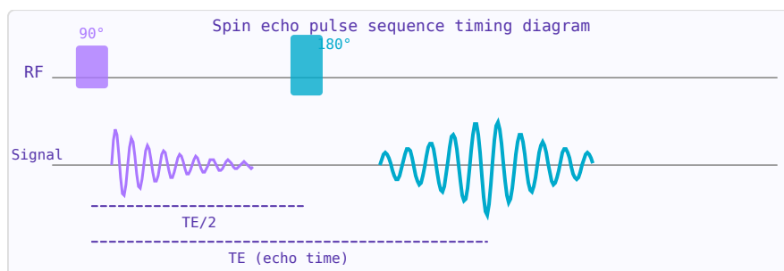
Figure 53.2: Spin echo: 90^\circ excitation creates FID (purple); 180^\circ refocusing pulse at TE/2 forms a spin echo at TE (cyan).
