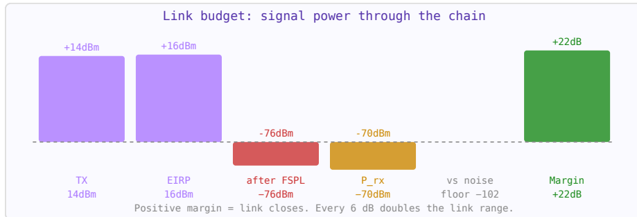
Figure 45.1: Link budget bar chart: TX power flows through gains and losses. Green margin bar = working link.
