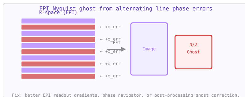
Figure 55.1: EPI Nyquist ghost: alternating k-space lines have opposite phase errors, creating a N/2 -shifted ghost image.
