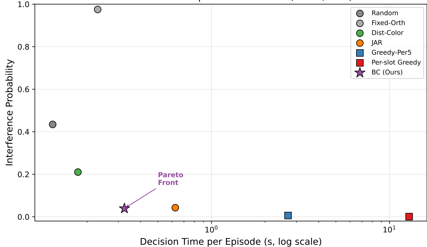
Performance-Computation Trade-off (N=10, v=0)
