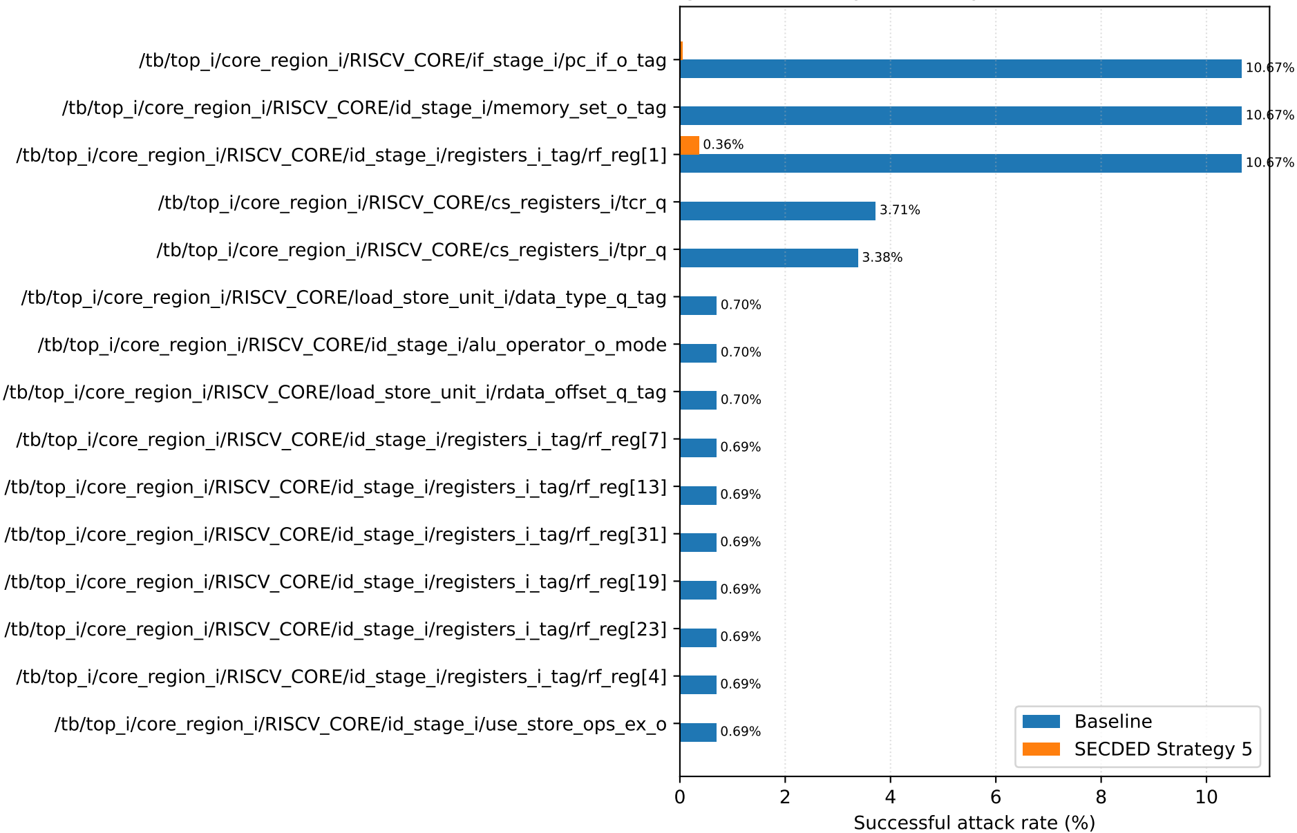
Register sensitivity ranked by Baseline — Buffer Overflow
