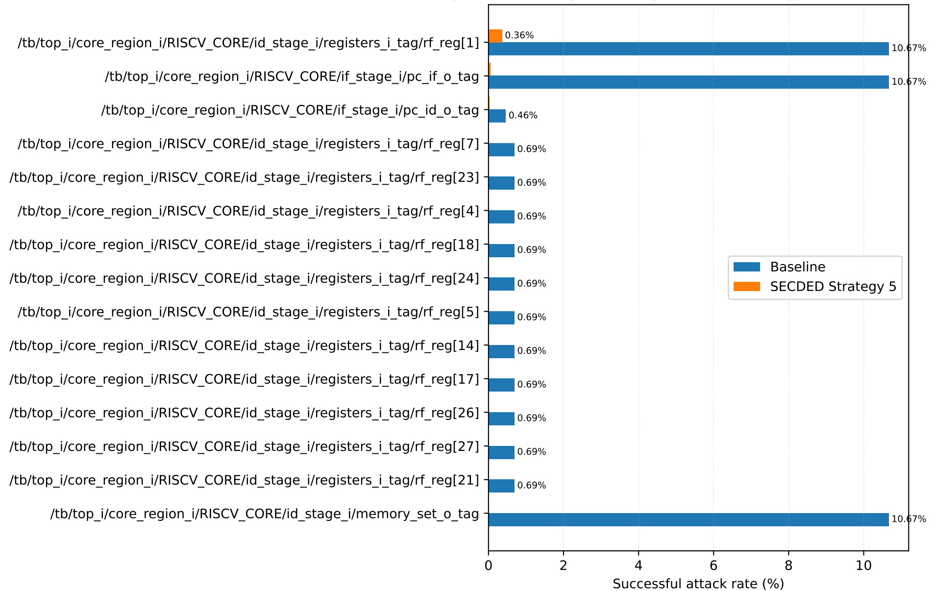
Register sensitivity ranked by SECDDED Strategy 5 — Buffer Overflow
