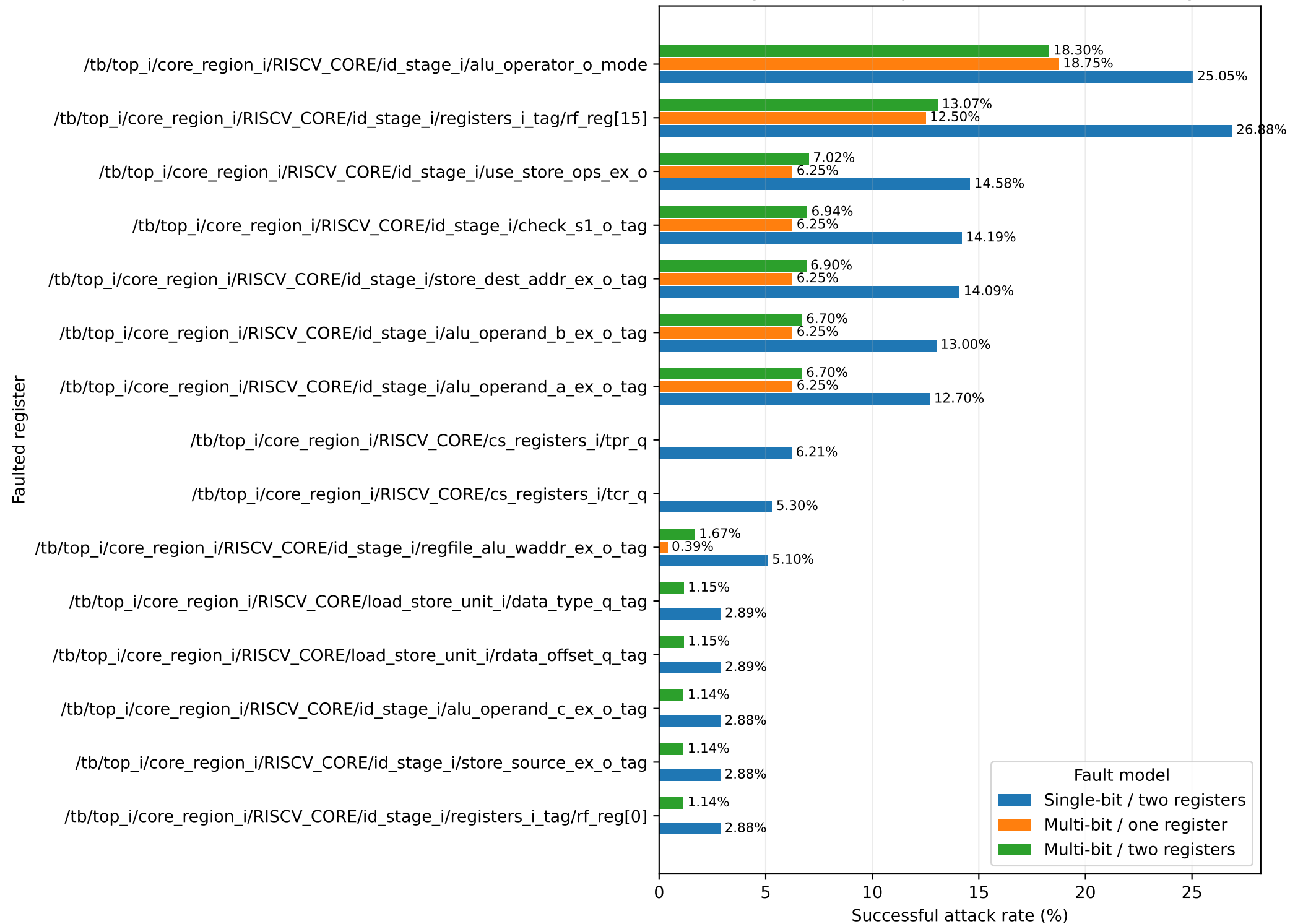
Register sensitivity — Baseline — Format String
