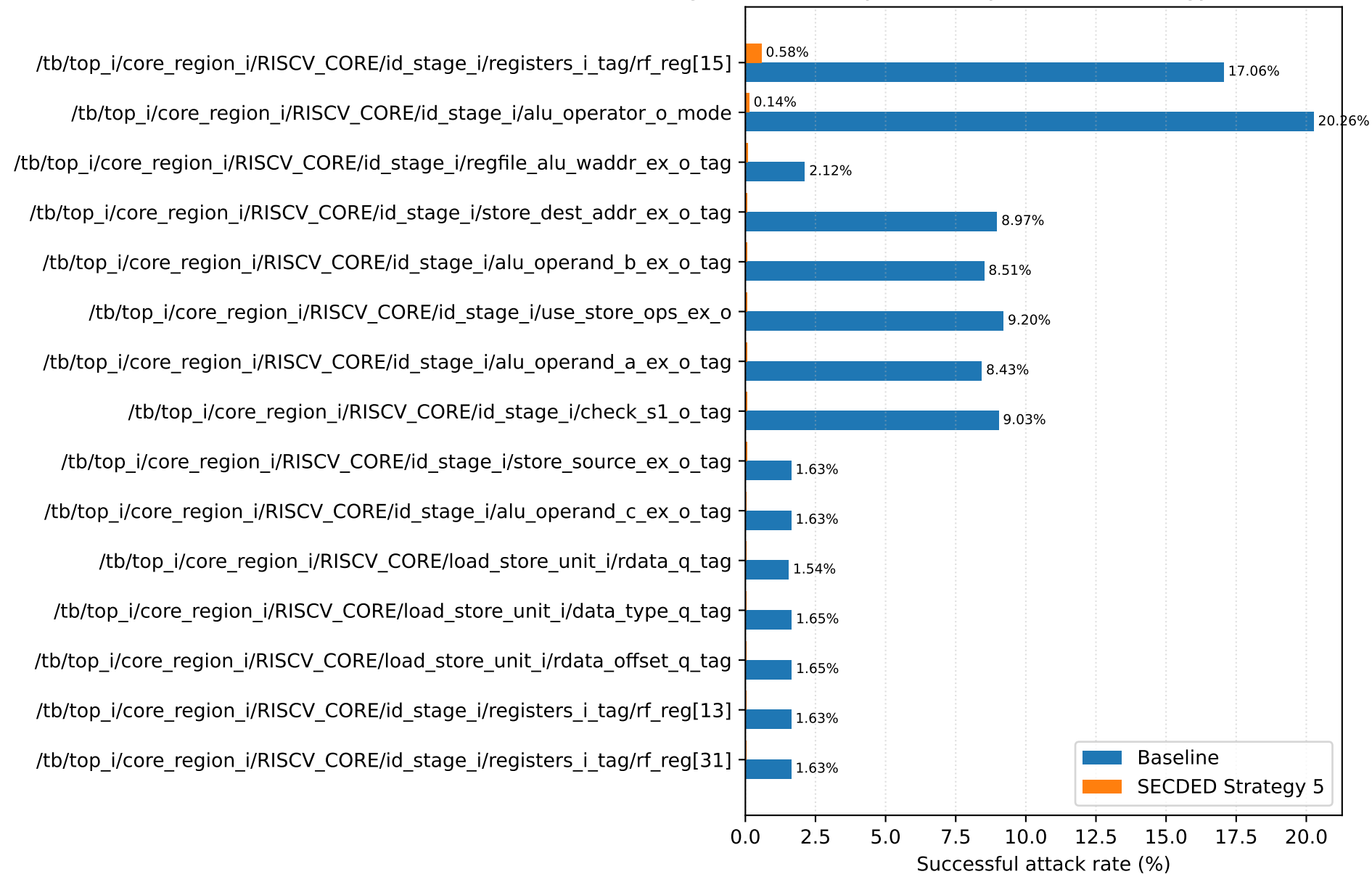
Register sensitivity ranked by SECDDED Strategy 5 — Format String
